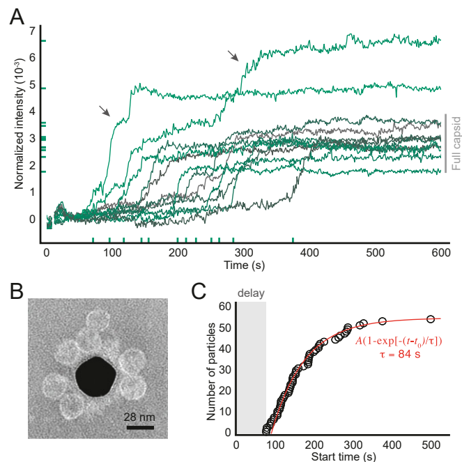
Fig. 2. Assembly of 2- \mu M coat-protein dimers around surface-tethered RNA strands. (A) Intensity traces for 12 randomly chosen particles from one experiment. x-axis ticks show the start times and y-axis ticks the final intensities. Gray bar indicates the intensity range corresponding to wild-type capsids. Arrows show 2 traces corresponding to overgrown particles. (B) Negatively stained TEM image of particles assembled around RNA strands tethered to a gold nanoparticle (dark region at center). We use a nanoparticle as the substrate because TEM cannot image through a coverslip. (C) The cumulative distribution of start times of all of the traces in the experiment is well fitted by an exponential with delay time t_0 of 92 s and a characteristic time \tau of 84 s (see SI Appendix for fit results from repeated experiments). Uncertainties in the start times are smaller than the diameter of the circles.
