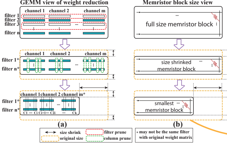
Figure 3: Structured weight pruning and reduction of hardware resources
