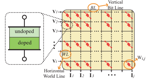
Figure 1: memristor and memristor crossbar field, which leads to the (memristance) state drift. Consequently, an error will incur when the state of memristor drifts to another state level.
