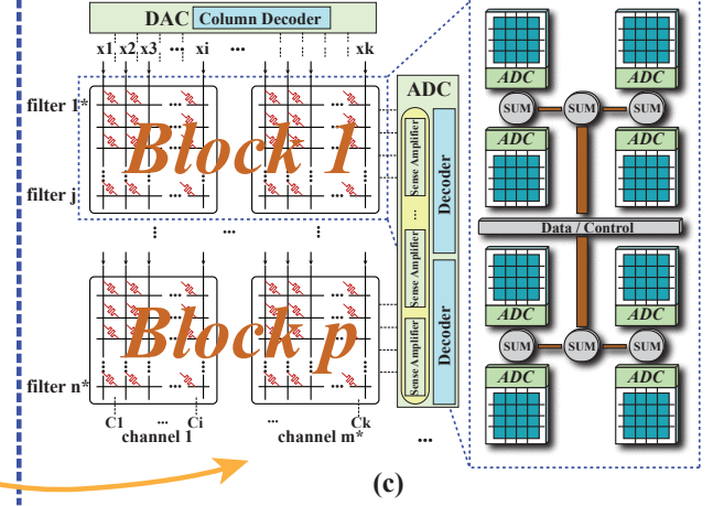
Figure 3: Structured weight pruning and reduction of hardware resources
