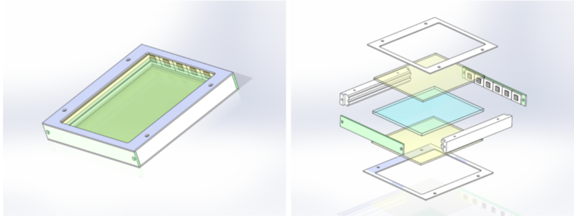
Figure 3.5. Left: an X-ARAPUCA cell. Right: an exploded view of the X-ARAPUCA cell, where the blue sheet is the WLS plate and the yellow sheets are the dichroic filters.
