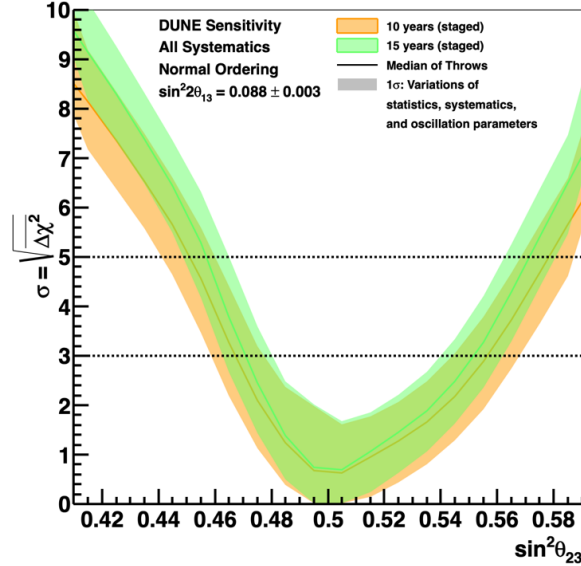
Figure 2.12. Sensitivity to determination of the \theta_{23} octant as a function of the true value of \sin^2 \theta_{23} , for ten (orange) and fifteen (green) years of exposure. True normal ordering is assumed. The width of the transparent bands cover 68% of fits in which random throws are used to simulate statistical variations and select true values of the oscillation and systematic uncertainty parameters, constrained by pre-fit uncertainties. The solid lines show the median sensitivity.
