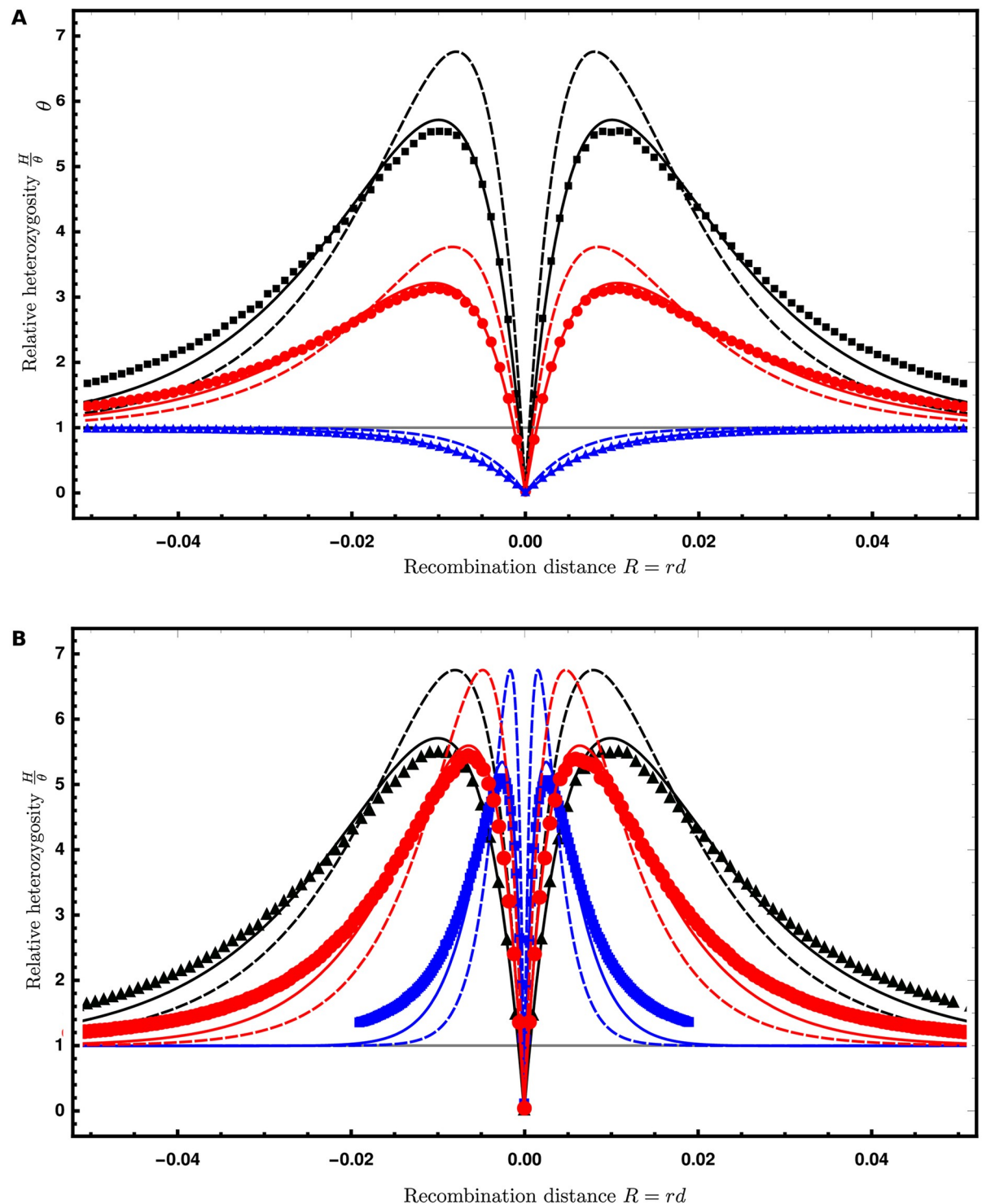
Fig 2. Volcanoes of diversity. Expected genetic diversity after the sweep relative to the initial heterozygosity, \frac{H}{H_0} , for a beneficial mutation centered at 0 as a function of the recombination distance R = rd to a neutral locus on left (–) and right (+) sides. For both panels, the lines show the predictions under the star-like approximation (dashed) and the better approximation (solid, see S1 Appendix, Section 1). The dots show the average \pm 3 standard errors about the mean (the error bars are smaller than the plot points). A. The effect of divergence of the donor population for an introgression sweep with 2Ns = 1000 . The divergence time (in units of 4N generations) is T_d = 6 (i.e., D = 13\theta , black), 3 ( D = 7\theta , red), and 0 ( D = \theta , blue), where T_d = 0 is a classic sweep from a de novo mutation. B. The effect of the strength of selection for an introgression sweep with T_d = 6 ( D = 13\theta ). The strength of selection is 2Ns = 1000 (black), 600 (red), or 200 (blue). For both panels, \theta = 0.002 ( N = 5000 , \mu = 10^{-7} ), r = 10^{-7} , and the window size is 100 nt.
