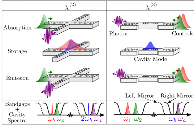
FIG. 1. Absorption, storage, and emission process with schematic illustrations of cavity implementations in \chi^{(2)} (left) and \chi^{(3)} (right) materials. Two sets of photonic crystal mirrors oriented perpendicularly ( \chi^{(2)} ) or inline ( \chi^{(3)} ) have band gaps in different frequency ranges as illustrated by the black lines in the bottom panel. One-sided cavities required for complete absorption are achieved by a slight frequency offset between the band gaps of the right (solid black) and left (dashed black) mirror. The decoupled mode (blue) is within the band gap of both mirrors while the coupled mode (purple) lies at the band edge of the left mirror. Only the decoupled cavity modes must have small volumes for efficient photon-photon interaction. The control modes are confined by weak mirrors ( \omega_1 and \omega_2 ) located at the exterior of the small cavity modes.
