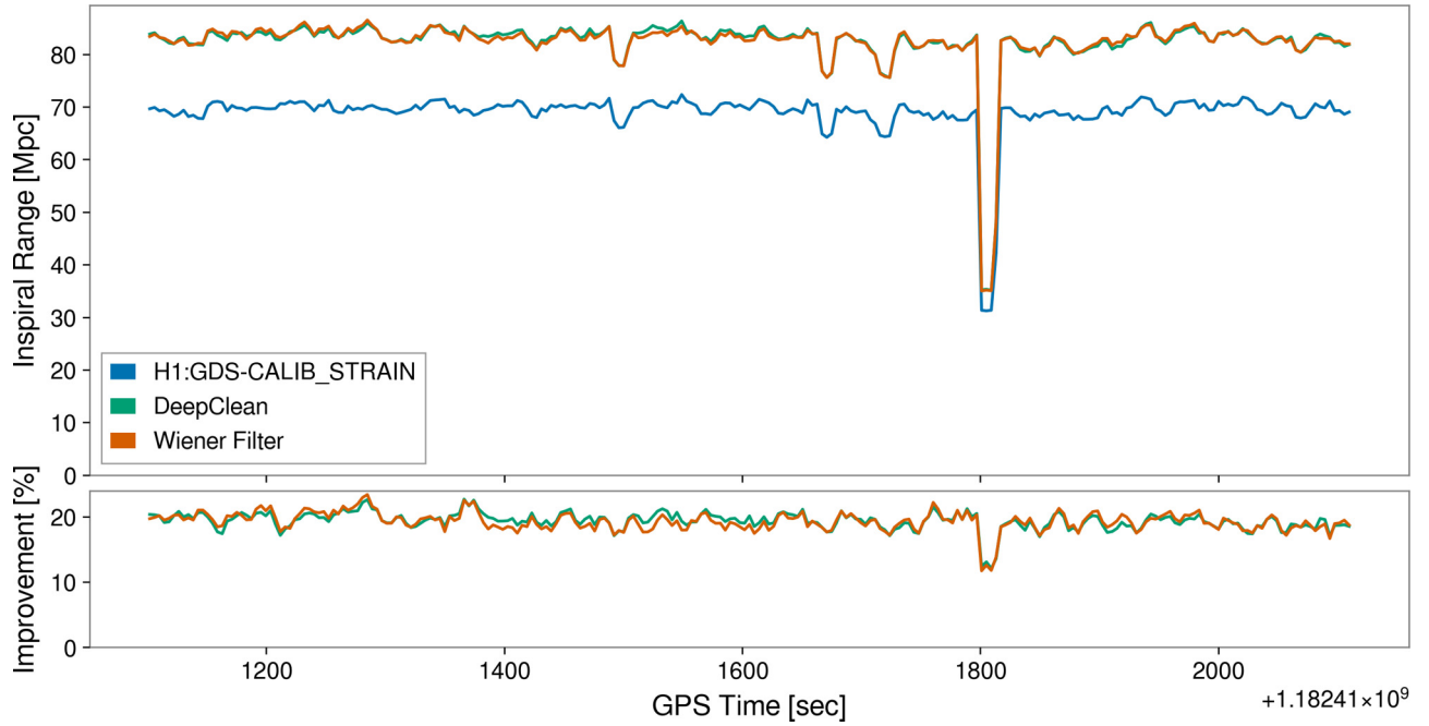
FIG. 4. The increase in the binary neutron star inspiral range after the linear subtraction is seen to be \approx 20\% .
