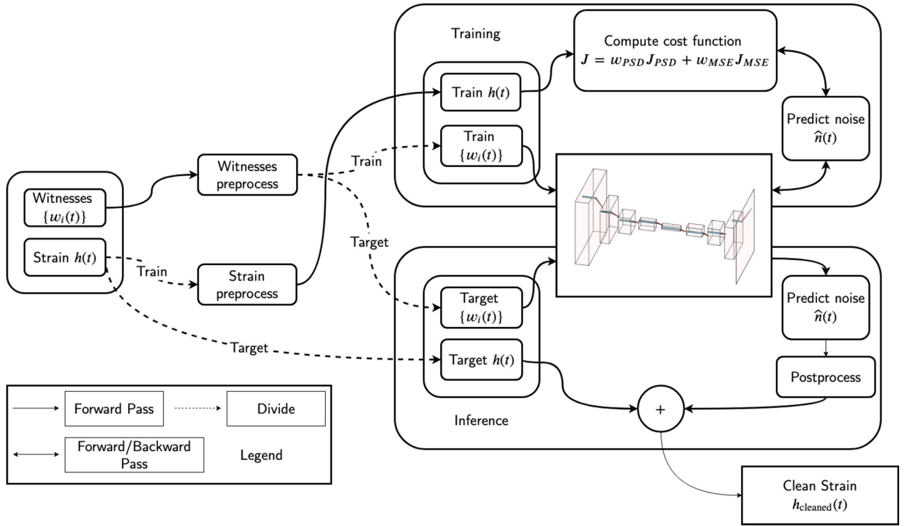
FIG. 2. Workflow diagram of the noise subtraction pipeline.
