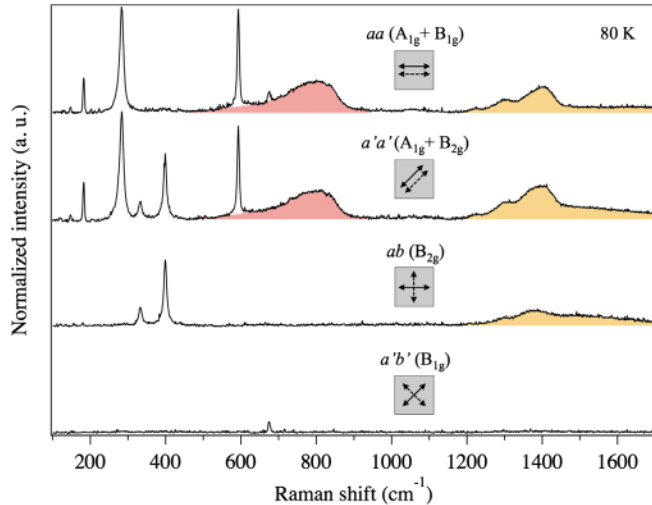
FIG. 3. Symmetry selection rules for the magnetic excitations in Sr 3 Ir 2 O 7 . Raman spectra were taken at 80 K in four polarization channels: aa , a'a' , ab , and a'b' . The insets indicate the polarization channels and the selected symmetry modes under the D_{4h} point group.
