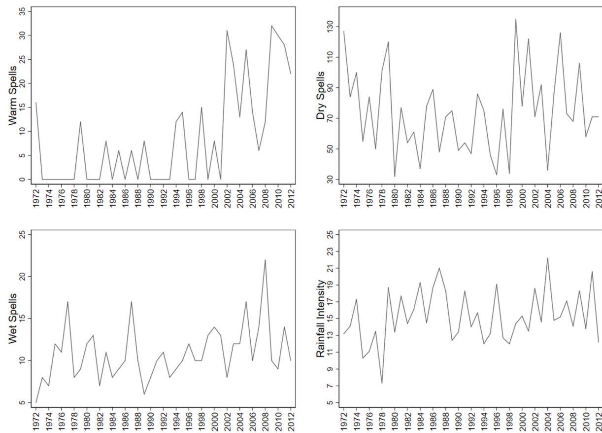
Figure 3. Observed values of four ETCCDI indicators, 1972 – 2012.
