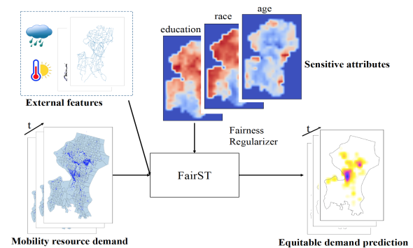
Figure 1: FairST is a Fairness-aware Spatial-Temporal model for new mobility systems. By incorporating a fairness regularizer, it makes equitable demand predictions between groups defined by, for example, race, age, or education level.
