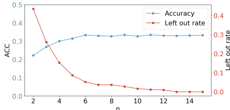
Figure 4: Experimental results on hyperparameter n . When n is larger than 6, selection of n does not affect the accuracy of the model.
