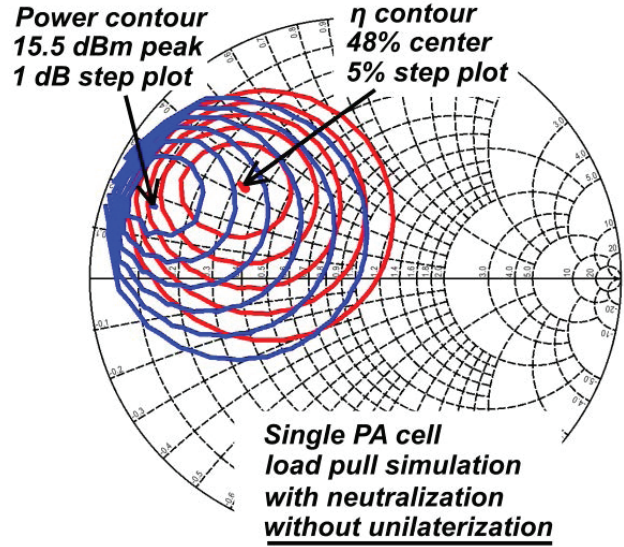
Fig. 11. Load-pull simulation of PA cell without unilateralization.
