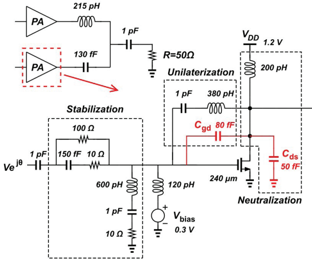
Fig. 10. Schematic of the proposed OPA with the neutralization, unilateralization, and stabilization networks.
