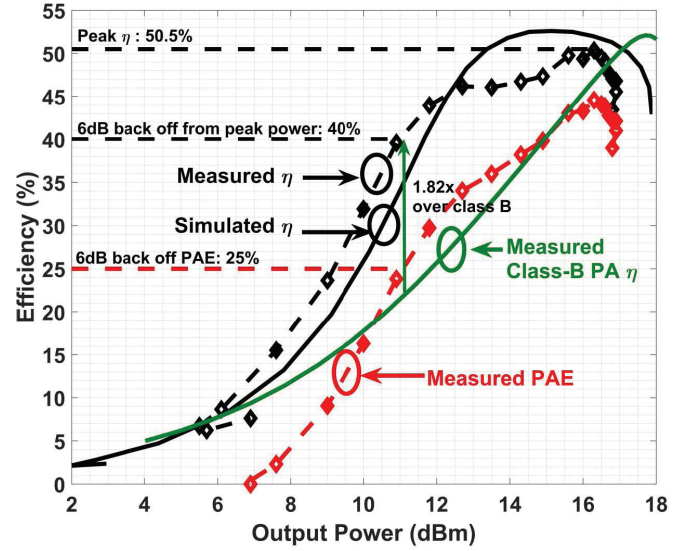
Fig. 18. Measured efficiency result comparing with simulation.
