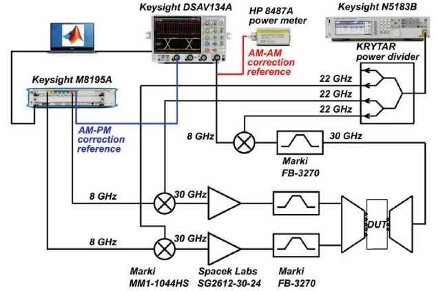
Fig. 19. Measurement setup.
