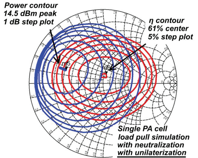
Fig. 12. Load-pull simulation of PA cell with unilateralization.
