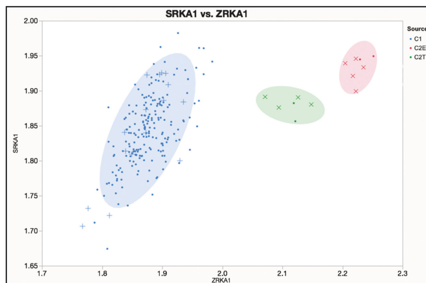
Figure 2. Bivariate plot illustrating archaeological samples (dots) and geological sources (plus signs (+), Carpathian 1 sources are blue plus signs (+), Carpathian 2E are red x's, and Carpathian 2T are green x's. The results are logged and ellipses represent 90% confidence intervals.
