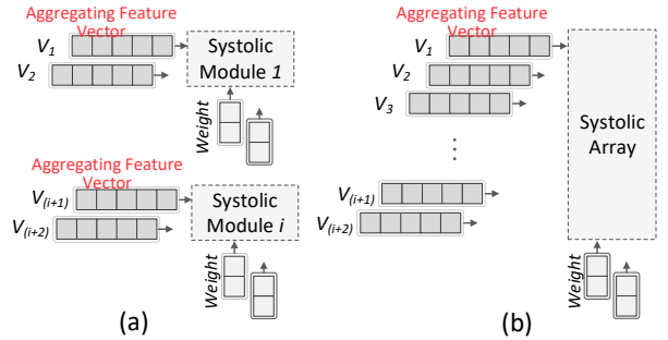
Figure 7. Different use of the systolic arrays: (a) independent working mode; (b) cooperative working mode.
