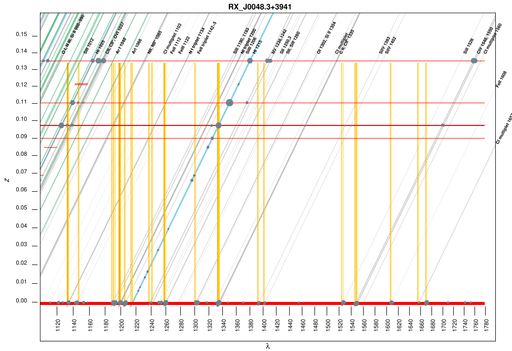
Figure B1. Example of conflict plot used to determine potential contamination in the velocity range -700 \lesssim v_{\text{LSR}} \lesssim -150 \text{ km s}^{-1} . Locations on the x -axis are scaled according to \log \lambda_{\text{obs}} , but the markers show the wavelength. The y -axis scale is proportional to \log(1+z) , but the markers show z . The diagonal lines represent loci of different transitions and how their observed wavelengths change with z . The gray lines correspond to metal transitions, while the green ones indicate \text{H}_2 transitions. Lyman series lines of H I are shown in blue. Some of the transitions are identified near the top and on the sides of the plot. Absorption features identified in the UV spectrum are shown with gray filled circles, with varying sizes proportional to \sqrt{W_\lambda} . The red horizontal lines represent redshift systems with any line (usually \text{Ly}\alpha ) that has W_\lambda \geq 100 \text{ mÅ} ; systems with \text{Ly}\alpha having strengths below this threshold do not have lines that stretch across the whole plot, but they do have short line segments that cover just \text{Ly}\beta and \text{Ly}\gamma . Most of the lines of interest appear along the yellow and orange lines, which represent a blueshift of -500 and -150 \text{ km s}^{-1} , respectively. Potential conflicts arise at the intersection of the horizontal red line, a gray/green/blue sloping line, and the vertical orange/yellow line.
