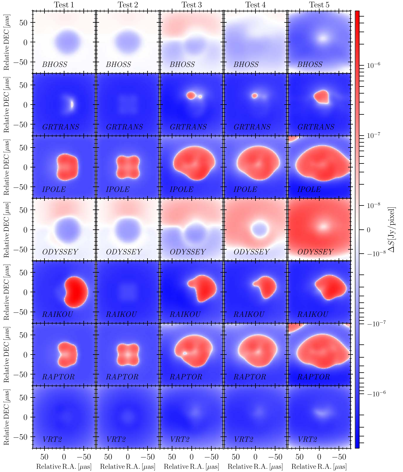
Figure 3. Difference images of the proposed test cases showing differences to the exact solution in janskys after convolving with the beam for different codes (from top to bottom) BHOS, GRTRANS, IPOLE/IBOTHROS, ODYSSEY, RAIKOU (来光), RAPTOR, and VRT2. White represents perfect agreement, blue indicates lower, and red indicates higher flux than the exact solution.
