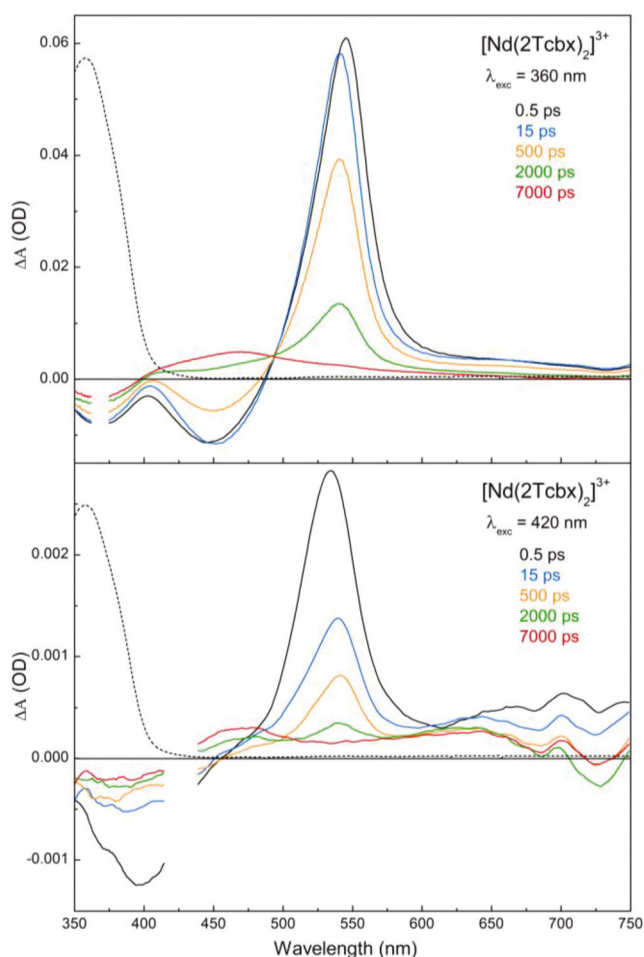
Fig. 5 (Top) Transient spectra of [Nd(2Tcbx) 2 ] 3+ collected with 360 nm excitation with different pump probe time delays. Inset legend assigns time delay with coloured trace. (Bottom) Transient spectra of [Nd(2Tcbx) 2 ] 3+ collected with 420 nm excitation with different pump probe time delays. Inset legend assigns time delay with coloured trace. The ground state spectrum of [Nd(2Tcbx) 2 ] 3+ is represented by the dashed trace in both plots.
