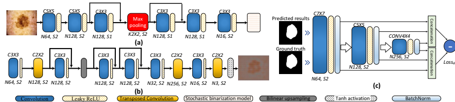
Fig. 2. Illustrations of (a) Compression network; (b) Feature reconstruction layers and (c) Discriminator network in our design.
