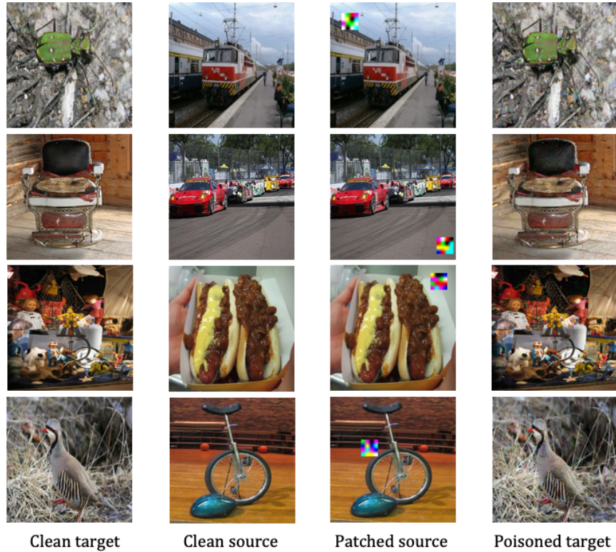
Figure 3: Visualization of target, source, patched source, and poisoned target images from different ImageNet pairs. For each row, the image in the fourth column is visually similar to the image in the first column, but is close to the image in the third column in the feature space. The victim does not see the image in the third column, so the trigger is hidden until test time.
