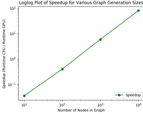
Fig. 4. A plot of the speedup of the GPU-accelerated version with respect to the CPU version of the modified PRM algorithm.
