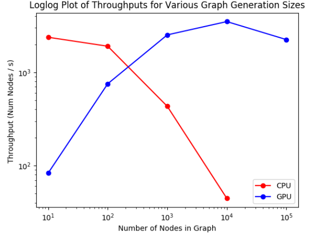
Fig. 3. A plot of the throughput of both the CPU and GPU-accelerated version of the modified PRM algorithm. Throughput is calculated by taking the number of nodes in the graph divided by the runtime.
