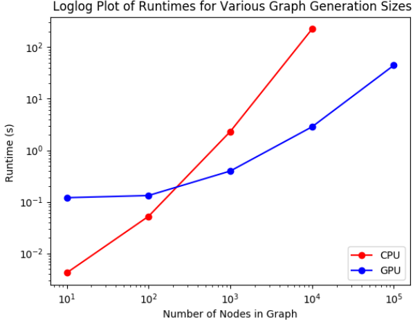
Fig. 2. A plot of the runtime in seconds of both the CPU and GPU-accelerated version of the modified PRM algorithm.
