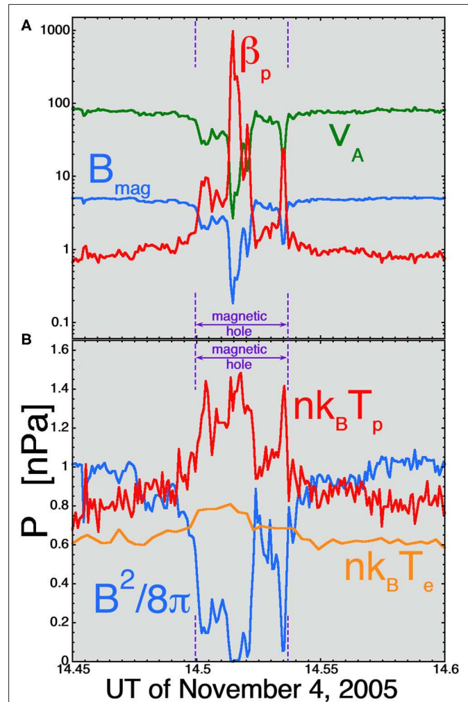
FIGURE 3 | An example of a magnetic hole (denoted in purple) during Flatop 15. Nine minutes of WIND spacecraft data [plasma properties in panel (A) and pressures in panel (B)] are plotted, and the duration of the magnetic hole as seen by WIND was 130 s.
