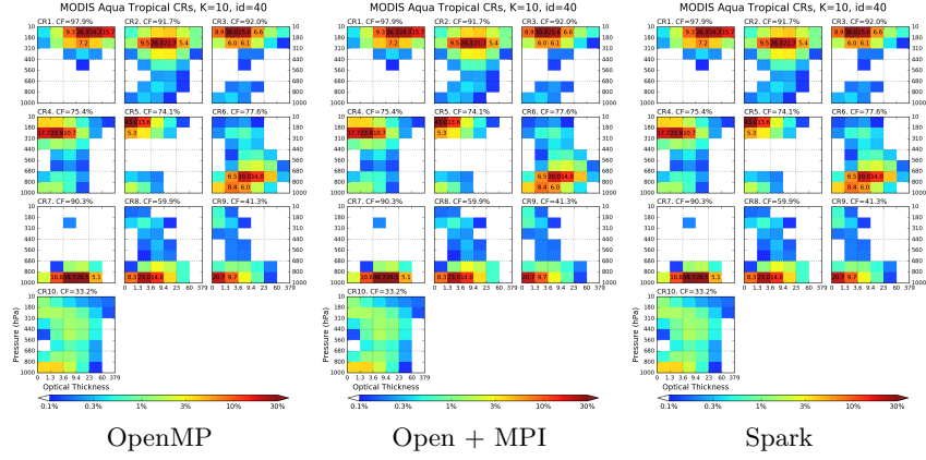
Fig. 4. Post-processed joint histogram results of the k-means final stable clusters for all three implementations. The images are qualitatively identical histogram model as discussed in [13]. This means that the scale, color, shape, and ordering of the histograms play an integral role in determining the accuracy of the implementation compared to the original.
