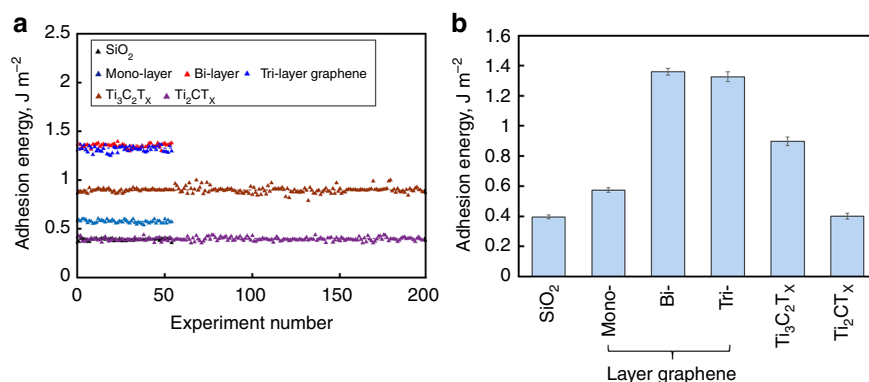
Fig. 5 a Adhesion energy for all measured samples (since adhesion energy of Ti 3 C 2 T x and Ti 2 CT x thin films is independent of the film thickness, MXene films with different number of monolayers are represented by one symbol in the graph), b average adhesion energies with error bars indicating standard deviations
