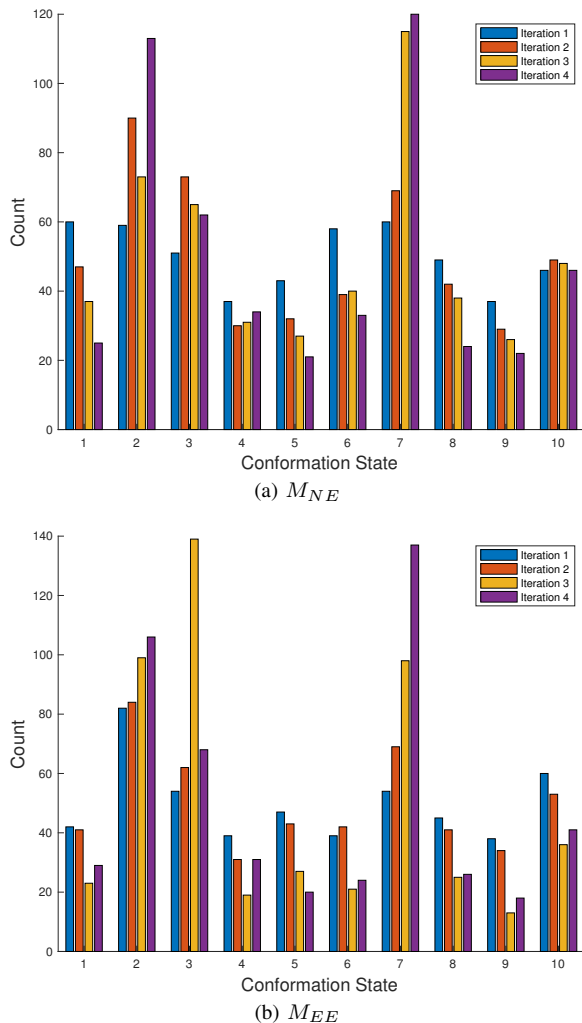
Fig. 6: Composition of ligand conformation states accepted for each iteration of (a) M_{NE} and (b) M_{EE} path optimizations (500 each iteration). State ‘1’ is the native conformation state and ‘2’–‘10’ are the non-native ligand conformation states. Some iterations showed a heavy preference towards particular conformation states, particularly states ‘2’, ‘3’, and ‘7’.
