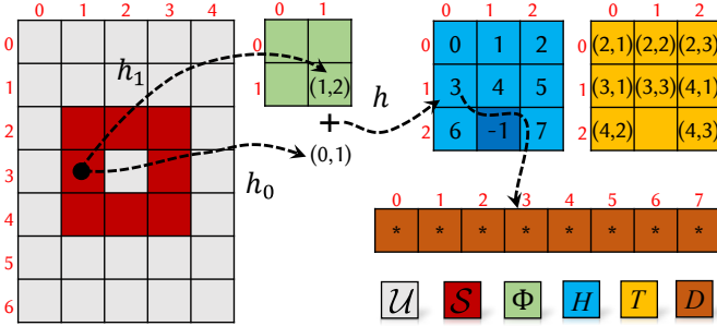
Fig. 3. An illustrative 2D example of the constitution of our PSH. The domain \mathcal{U} consists of 7 \times 5 2D voxels or pixels. The red-shaded pixels stand for the input model. The green, blue, yellow and brown tables are the offset table ( \Phi ), hash table ( H ), position tag ( T ) and data array ( D ) respectively.
