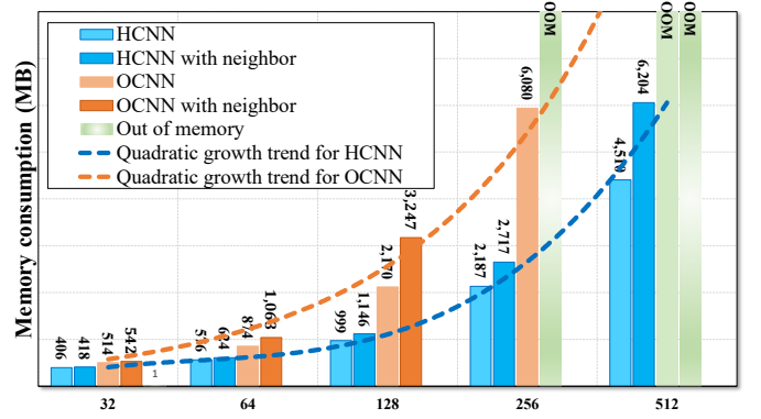
Fig. 7. The actual memory consumption using OCN and HCNN over a mini-batch of 32 models. The physical memory cap of the 1080 GTX card is 8 GB. HCNN allows very dense voxelization up to 512^3 even with pre-stored neighbor information, while OCN can only handle resolution of 128^3 with recorded neighborhood.
