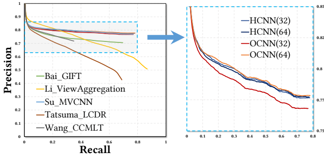
Fig. 8. The precision recall curves for HCNN, OCNN as well as other five famous multi-view CNN methods from SHREC16. The difference between HCNN and OCNN (under resolutions of 32^3 and 64^3 ) is quite subtle even after zooming in.
