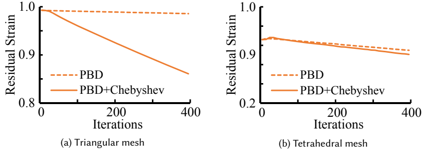
Fig. 7. The convergence of position-based dynamics, using Jacobi iterations. This example shows that the acceleration effect of the Chebyshev approach is more significant on triangular meshes as shown in (a) than on tetrahedral meshes as shown in (b).
