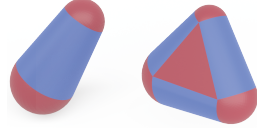
Fig. 3. Linearly interpolating medial spheres over an edge or a triangle yields a medial cone (left) or a medial slab (right).
