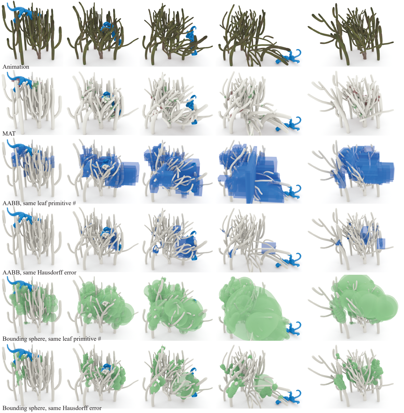
Fig. 15. The dinosaur model falls through a group of eight cacti. We compare our MAT-based CC with BVHs of AABBs and bounding spheres. This animation runs at \sim 18 FPS with all the collisions and self-collisions culled, detected, and resolved. MAT-based CC/SCC is highlighted in the second row, where the deformed MATs of all the cacti are also given. For BVHs of AABBs and spheres, we either set the BVH to have the same bounding quality as MAT (same Hausdorff error) or to have the same number of leaf primitives as MPs on the MAT (same leaf primitive #). Only leaf-level AABBs and spheres are highlighted.
