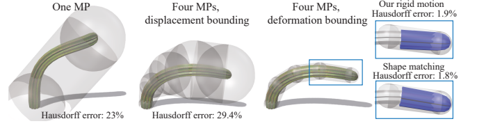
Fig. 7. Displacement bounding scales medial spheres based on vertices' displacement of the MP. As long as the model deviates far from its rest shape, displacement bounding produces a loose enclosure even with little deformation. Deformation bounding fixes this issue by computing a local generalized coordinate with rigid drift factored out.
