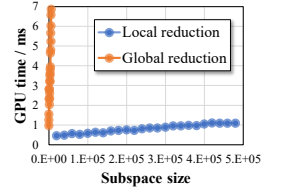
Fig. 5. The local step is sublinear w.r.t. subspace dimension. Projecting 500,000 as-rigid-as-possible constraints only takes 1.1 ms on the Titan GPU. Global step needs to solve a linear system and is more sensitive to the problem size.
