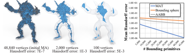
Fig. 2. Volumetric MAT approximation of the Armadillo model (with 62, 161 surface triangles). The initial MA (the leftmost subfigure) contains around 50k medial vertices. After aggressively simplifying the MM to only 100 vertices, the mean Hausdorff error remains less than 1%. Note that the vertical axis of the rightmost plot is logarithmic.
