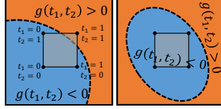
Fig. 9. Two medial cones intersect when g(t_1, t_2) = 0 overlaps with the constraint region (left), or one medial cone is completely inside of the other (right).
