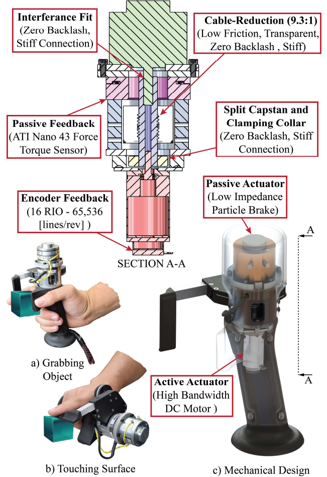
Figure 6. Two haptic interactions enabled by the handheld haptic device. a) Grabbing a virtual object. b) Touching a surface. c) Low impedance mechanical design of the hybrid actuator enabling a transparent rendering.
