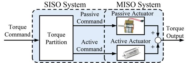
Figure 2. Generalized control topology of a multi-input single output hybrid actuator recast into a single input single output system.
