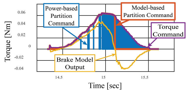
Figure 4. Time domain plot of the torque command by our model-based passive partitioning method compared to results obtained by power-based partitioning. The figure also shows the time domain results of the Dahl inspired model.
