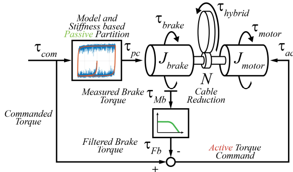
Figure 1. Hybrid actuation approach model and signal flow diagram.
