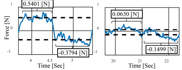
a) Measured Output - No Control b) Measured Force - Hybrid Control
