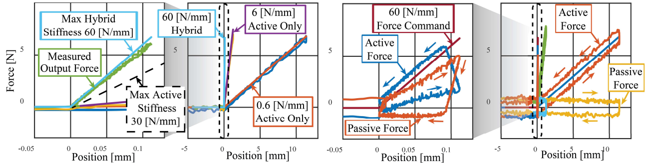
a) Zoomed 60 [N/mm] hybrid rendering b) Virtual wall comparison c) Hybrid torque contributions d) Low stiffness active and passive torques Figure 7. Various rendering stiffness, 60 [N/mm], and two lower stiffness, 6 [N/mm] and 0.6 [n/mm], left to right respectively. The sample frequency is set at 5000 [Hz] for all tests. a) Maximum hybrid stiffness with measured output force. b) Virtual wall comparison with measured output force. c) Active and passive contributions to the 60[N/mm] hybrid virtual wall. d) Active command and measured passive torque contributions at lower stiffness.
