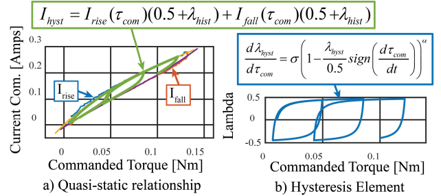
Figure 12 a) Quasi-static steady state torque current relationship. With third order polynomials I_{rise} and I_{fall} b) Hysteresis element (lambda) forming minor loops of rate independent hysteresis behavior.
