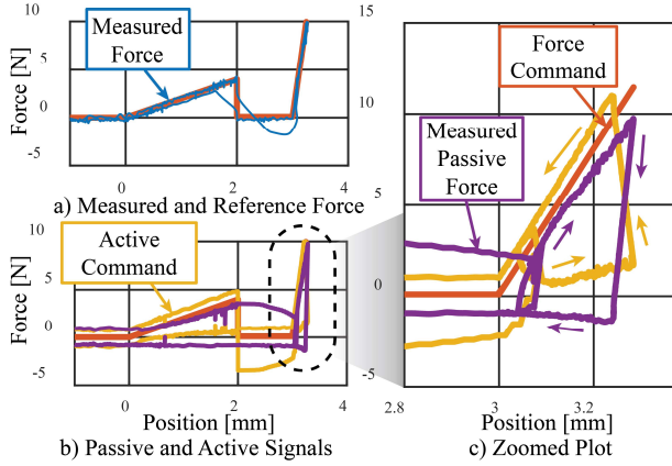
Figure 10. Hybrid rendering of a button K1 = 2\text{N/mm} Fr = 0.1 K2 = 40\text{N/mm} m = 2\text{mm} n = 3\text{mm} fs = 5000 [Hz] a) Compares measured Zero Lag Filtered (SOF 40Hz cutoff) output force (blue) and Reference torque (red) b) Shows the reference torque (red) and the measured filtered passive force (purple) and the commanded active torque (yellow) c) Is a zoomed plot of the stiff wall interaction at the end of the buttons throw.
