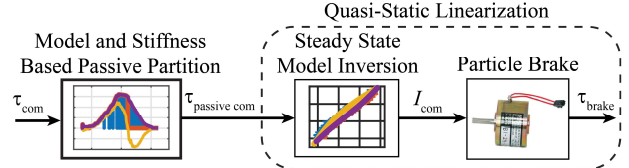
Figure 11. Block diagram showing quasi-static model inversion to improve steady state torque rendering accuracy, and the model based passive partition which includes electrical and mechanical dynamics.
