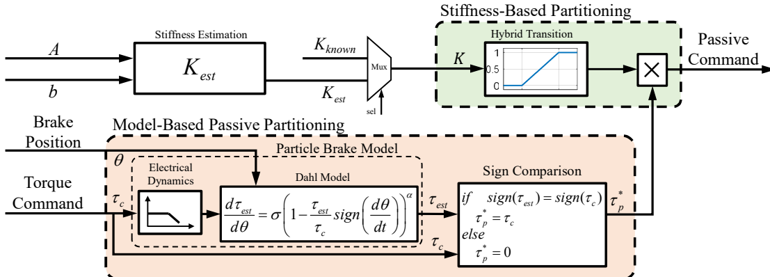
Figure 5. Passive partition including stiffness-based partitioning and model-based passive partitioning. Either a known or estimated stiffness might be used as the input signal for the hybrid transition. Additional information about the stiffness estimation method can be found in appendix B.
