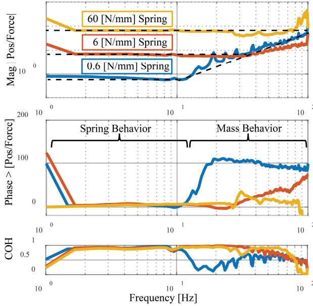
Figure 8. Magnitude, Phase, and Coherence of impedance frequency responses. A soft (0.6 [N/mm]), medium (6 [N/mm]), and stiff (60 [N/mm]), spring are shown in blue red and yellow respectively. A chirp is used to excite the system from 0.1 [Hz] to 100 [Hz]. A Hanning window, 50% overlap, and 199 frequency averages were taken [Hz] and the discrete control system is running at 5000 [Hz]
