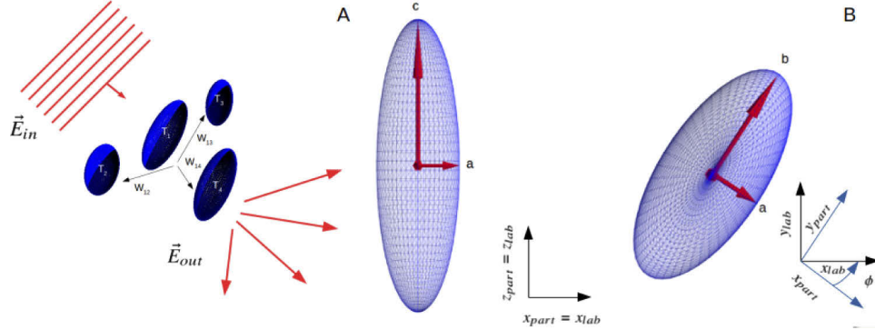
Fig. 1. A. Mie scattering schematic. Light is incident onto the set of ellipsoidal scatterers. Each scatterer has an associated T-matrix. The incident field onto each scatterer is described by the incident field E_{in} and the scattered fields from all other scatterers. The inter-particle coupling is represented by the matrix W_{n''n'} , which describes the coupling between spheres i' and i'' . B. Design parameters for ellipsoidal scatterers. The semi-major axes are taken to always be aligned with the particle frame: semi-major axis a is aligned with the x_{part} axis, b with the y_{part} axis, and c with the z_{part} axis. The rotation \phi is about the z -axis, with the counterclockwise direction defined as a positive rotation.
