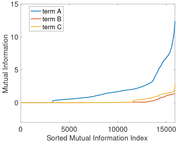
Fig. 8 Pairwise mutual information breakdown
