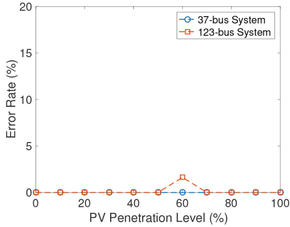
Fig. 16 ERs with different levels of DER penetration using |\Delta V^{pnz}|
