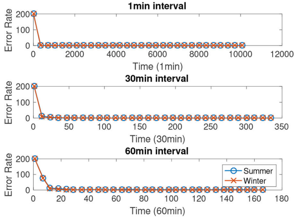
Fig. 18 ERs with summer and winter load patterns
