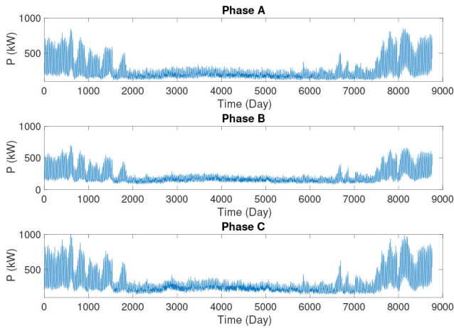
Fig. 14 Hourly aggregated real powers on each phase in 37-bus system
