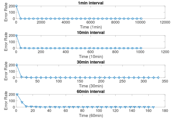
Fig. 20 ERs with different data resolutions
