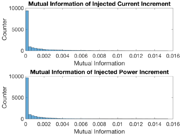
Fig. 2 Mutual information of pairwise current injection increment \Delta I and power injection increment \Delta S of PG&E data sets in the IEEE 123-bus system
