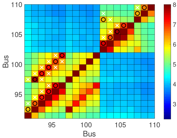
Fig. 6 Mutual information of pairwise buses in IEEE 123-bus system using PG&E data sets. The circle indicates the neighbours of bus i . The crossing indicates the two-step neighbour of bus i . The square without markers represents the bus pair that are more than two-step away
