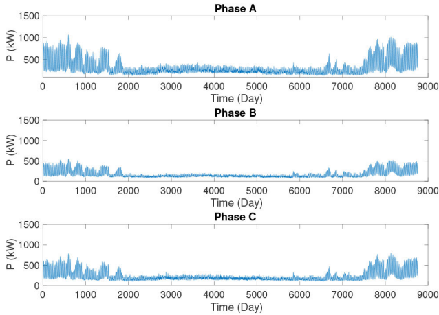
Fig. 15 Hourly aggregated real powers on each phase in 123-bus system
