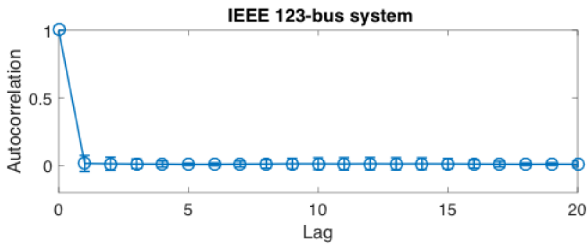
Fig. 3 Average auto-correlation of current injection increment \Delta I of PG&E data sets in the IEEE 123-bus system. The error bar is one standard deviation
