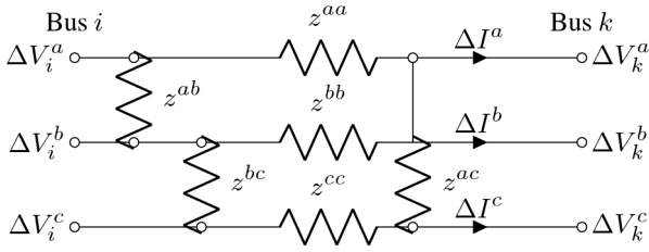
Fig. 10 Example of the two-port three-phase circuit
