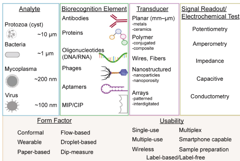
Fig. 1. Components and measurement formats associated with electrochemical biosensors for pathogen detection.
