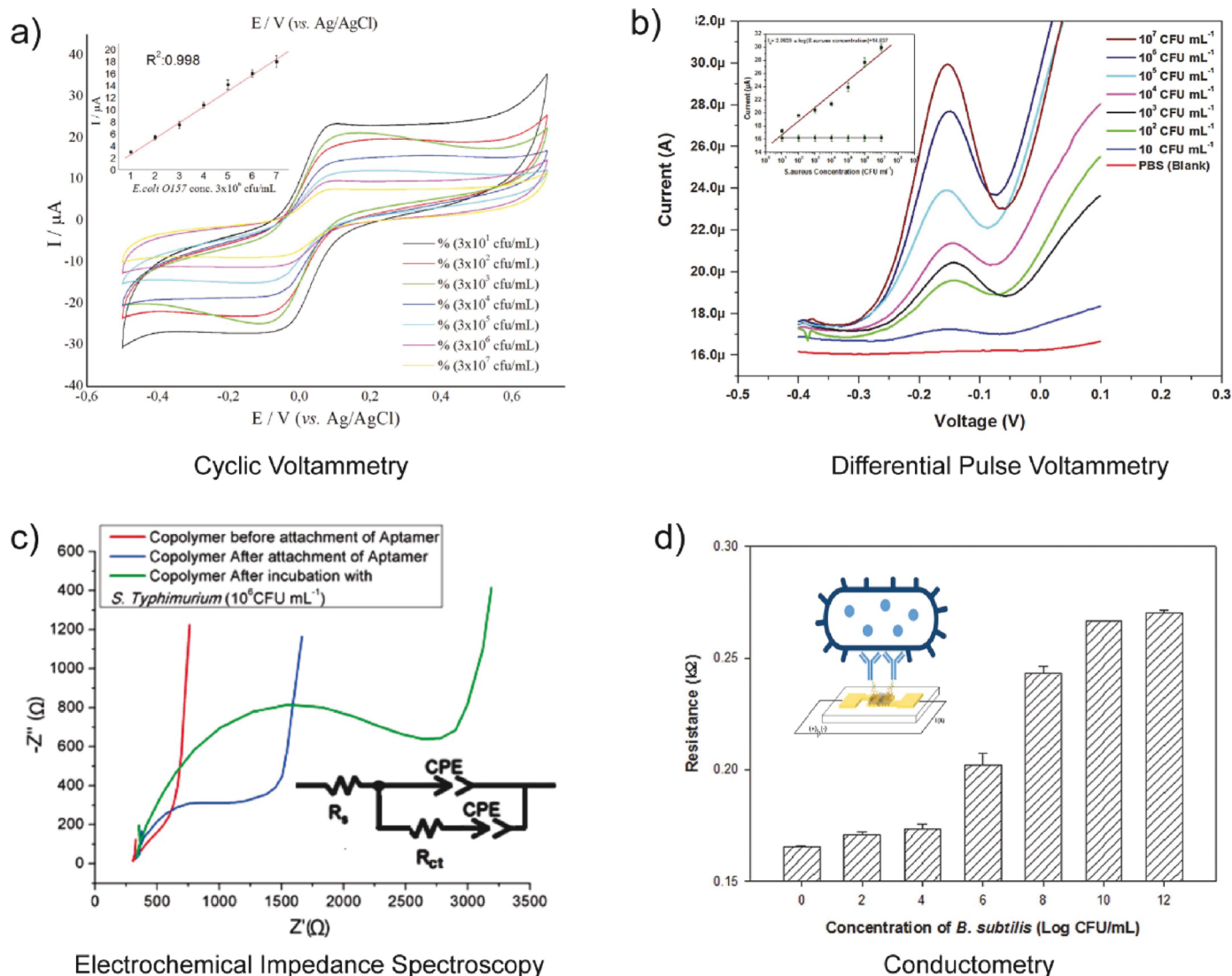
Fig. 5. Typical responses associated with the common electrochemical methods used for pathogen detection. a) Cyclic voltammetry (CV) data using Fe(CN)_6^{3-/4-} for varying concentrations of E. coli (Güner et al. 2017). b) Differential pulse voltammetry (DPV) data using Fe(CN)_6^{3-/4-} for varying concentrations of S. aureus (Bhardwaj et al. 2017). c) Electrochemical impedance spectroscopy (EIS) in 100 mM LiClO_4 solution in the form of a Nyquist plot and corresponding equivalent circuit model associated with biorecognition element immobilization and detection of S. typhimurium (Sheikhzadeh et al. 2016). d) Conductometry data for varying concentrations of B. subtilis (Yoo et al. 2017).
