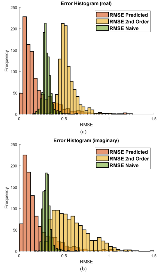
Fig. 3. Real (a) and imaginary (b) RMS error histograms for all 1000 validation problems. Predicted case is for the proposed macro basis function approach. Naïve case gives the error of the solutions directly predicted with the network using no macro basis function approach (the typical, existing approach). 2 nd -order case serves as a comparison to the proposed approach. The 2 nd -order case and predicted case use the same number of basis functions, but the proposed method yields error an order of magnitude lower.
