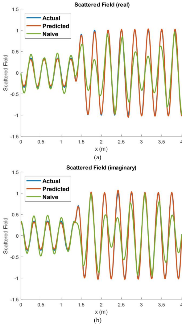
Fig. 2. Scattered field (z-directed) solution comparison between weak solution obtained using predicted macro basis functions, actual solution, and naïve predicted solution: (a) real component and (b) imaginary component. Naïve predicted solution is obtained by plotting the solution directly predicted by the network without the macro-basis function approach.
