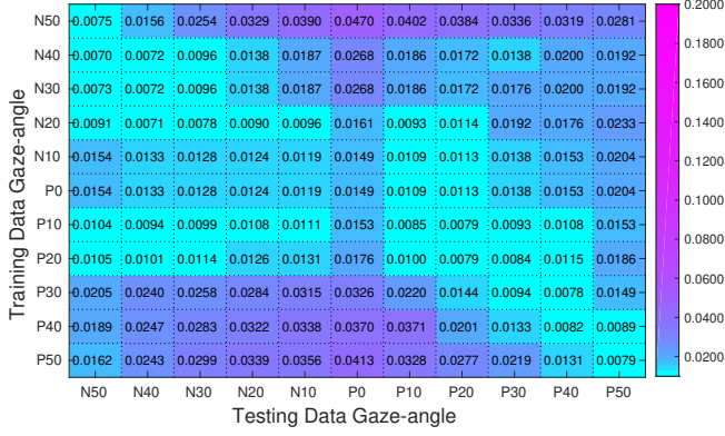
Figure 4: Segmentation performance of SegNet trained and tested on each gaze-angle separately as average nice1 error.
