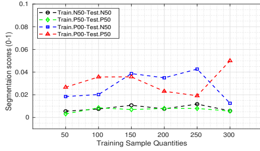
Figure 7: Segmentation performance of SegNet (average nice1 ), trained with increasing quantities of P0 gaze-angle images, on the N50 and P50 gaze-angles images vs. trained with identical (N50 and P50) gaze-angles images.
