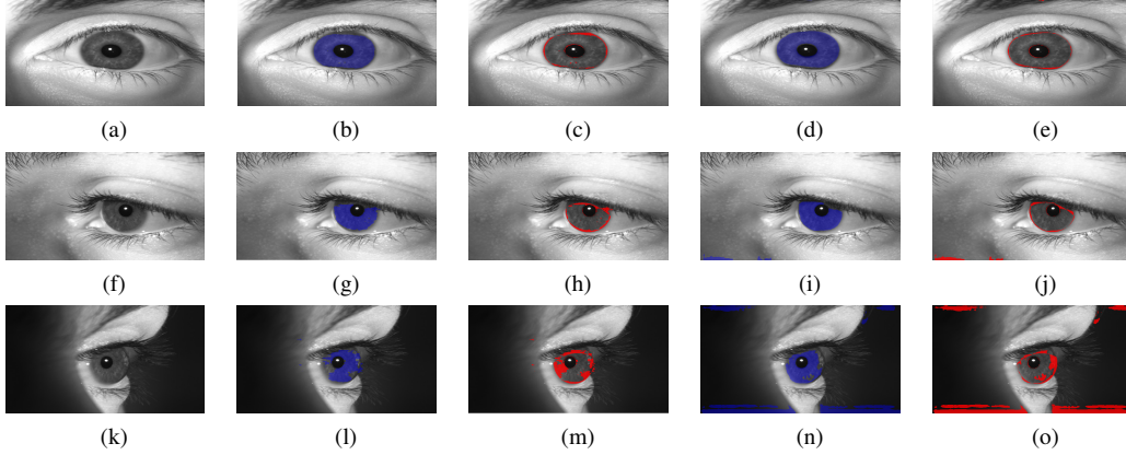
Figure 6: Sample iris images of P0 (6a), N50 (6f), and P50 (6k) gaze-angles in the database, and their corresponding segmentation (blue color) masks, and error (red color) masks using SeNet (second and third column), and RefineNet (fourth and fifth column), trained on frontal iris data, respectively.
