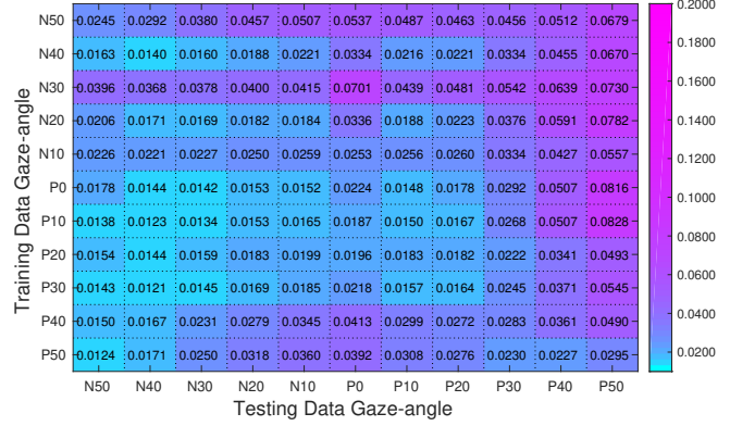
Figure 5: Segmentation performance of RefineNet trained and tested on each gaze-angle separately as average nice1 error.
