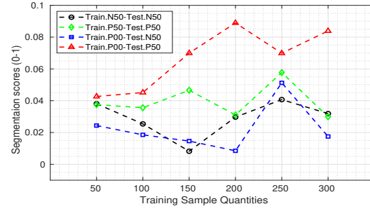
Figure 8: Segmentation performance of RefineNet (average nice1 ), trained with increasing quantities of P0 gaze-angle images, on the N50 and P50 gaze-angles images vs. trained with identical (N50 and P50) gaze-angles images.
