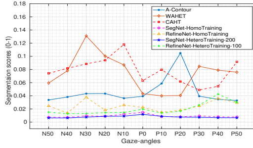
Figure 10: Segmentation performance of the CNN networks vs. classical methods’ performance as average nice1 error.
