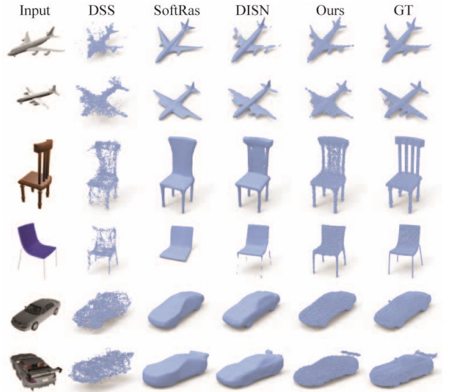
Figure 10. Qualitative comparison with differentiable renderers for different 3D representations and supervised learning methods.
