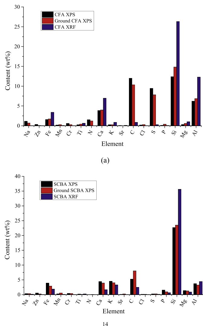
Fig. 4. Comparisons between the element proportions extracted from XRF and XPS tests: (a) CFA samples; (b) SCBA samples.
