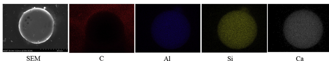
Fig. 9. SEM image of a CFA grain and element mappings based on EDS.
