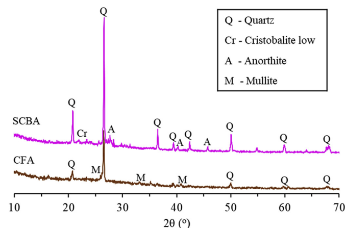
Fig. 2. XRD diffractograms of CFA and SCBA.
