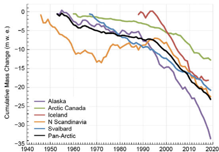
Fig. 5.17. Cumulative B_{\text{clim}} in meters of water equivalent (m w.e.) for monitored glaciers in five regions of the Arctic and for the Arctic as a whole (Pan-Arctic). Mean balances are calculated for glaciers monitored in each region in each year and these means are summed over the period of record. Note that monitoring periods vary between regions and that the number and identity of glaciers monitored in a given region may vary between years. (Source: WGMS 2017.)
