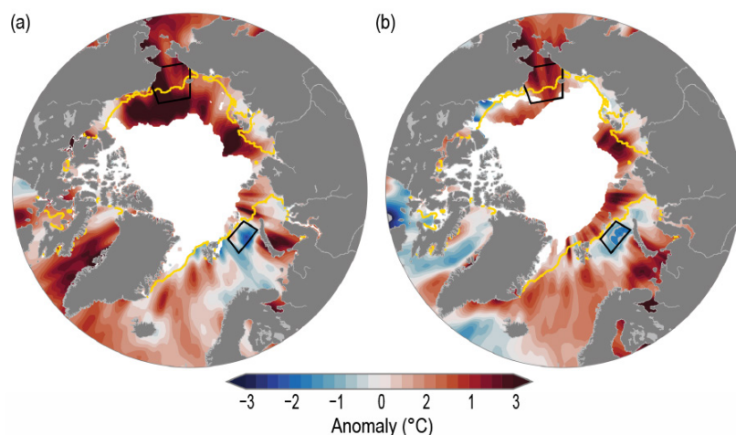
Fig. 5.5. SST anomalies ( ^{\circ}\text{C} ) in (a) Aug 2019 and (b) Aug 2018 relative to the Aug 1982–2010 mean. The yellow line indicates the median ice edge for Aug 1982–2010 and white shading indicates the mean sea ice extent in (a) Aug 2019 and (b) Aug 2018. The two regions marked by black boxes relate to data presented in Figs. 5.6 and 5.7. (Sources: SST data are from the NOAA OISSTv2; sea ice extent and ice-edge data are from NOAA/NSIDC Climate Data Record of Passive Microwave Sea Ice Concentration, Version 3; Peng et al. 2013; Meier et al. 2017.)
