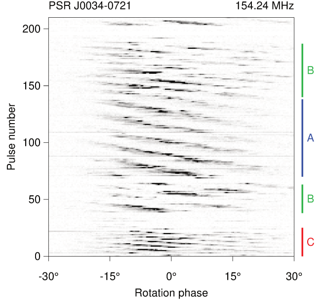
Figure 11. A sequence of 210 individual pulses from PSR J0034–0721 that shows the phenomenon of sub-pulse drifting. The observations were made with Phase II over the 140–170 MHz band, and processed using the newly-enhanced tied-array beam-former pipeline that resynthesises the VCS-recorded data to produce high-time resolution ( \sim 1 \mu\text{s} ) time series. The pulsar switches between three distinct drift bands (designated as Modes A, B and C) and exhibits the phenomenon of nulling (i.e. cessation of pulses) and is a promising target for studying emission mechanisms.
