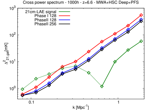
Figure 5. Expected sensitivity to the 21cm-LAE power spectrum at z=6.6 with an observation of 1000h, HSC and PFS survey. The signal is calculated by using large scale radiative transfer simulation of reionisation, which is identical to the simulation used in Kubota et al. (2018).
