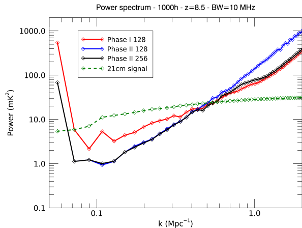
Figure 2. Typical EoR power spectrum model at 150 MHz with associated noise levels available to the Phase I and Phase II arrays with 1000 h observation. “Phase II 256” represents the result from a future MWA upgrade where all 256 tiles are used simultaneously. (From Wayth et al. 2018)
