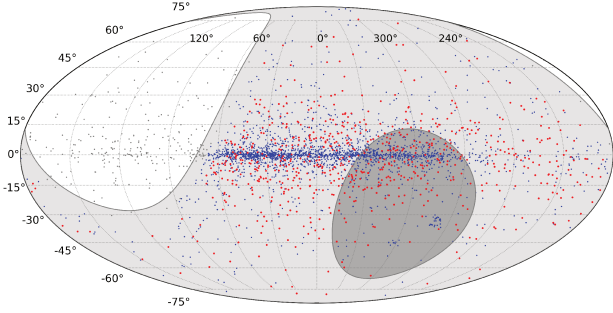
Figure 10. Simulated pulsar detections (red dots) from an all-sky high time resolution survey with the MWA. The grey region represents the MWA’s visible sky, and the dark-grey region the sky that is exclusively accessible by the MWA at frequencies below 300 MHz (declination < -55^\circ ). The blue dots are pulsars from the ATNF pulsar catalogue v1.59
