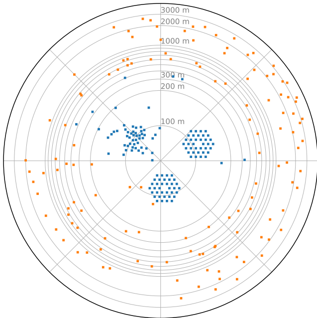
Figure 1. The compact and extended configurations of the Phase II MWA. The blue and orange squares show the tiles which are correlated in the compact and extended configurations respectively. Note the linear radial scale within 200 m to show the dense pseudo-random/redundant hybrid core, and logarithmic radial scale beyond to capture the nearly 6 km diameter.
