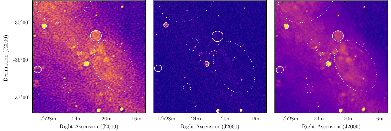
Figure 6. A region of sky centred on RA 17^{\text{h}}22^{\text{m}} , Dec -36^\circ at 139–170 MHz is shown using three different datasets and imaging techniques. Left: A single two-minute snapshot from the original Phase I configuration, imaged with multiscale WSCLEAN and a Briggs weighting of -1 (Hurley-Walker et al. 2019a, accepted); Middle: A single two-minute snapshot from the extended array, imaged with multiscale WSCLEAN and a Briggs weighting of 0; Right: The two observations imaged together using image-domain-gridding (van der Tol et al., 2018) in WSCLEAN and a Briggs weighting of 0. Known SNRs are shown with solid lines, while SNRs detected by Hurley-Walker et al. (2019b, accepted) are shown with dotted lines. The increased resolution and imaging quality of Phase II MWA make it possible to discern these SNRs in four minutes, instead of \approx 30 minutes.
