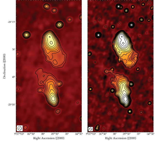
Figure 8. Images of ESO 422–G028 from Phase I (left, from GLEAM; Hurley-Walker et al. (2017)) and Phase II (right, from GLEAM-X, Hurley-Walker et al., in prep). Colour-scale and contours both denote the surface brightness at 200 MHz. Colour scale ranges from -3\sigma to 100\sigma on an arcsinh stretch to emphasise faint diffuse emission. Contours start at 3\sigma and scale by a factor \sqrt{2} , where \sigma = 14.9 \text{ mJy beam}^{-1} ( 2.0 \text{ mJy beam}^{-1} ) in the Phase I (Phase II) image. The beam size is shown by the hatched ellipse in the lower-left corner.
