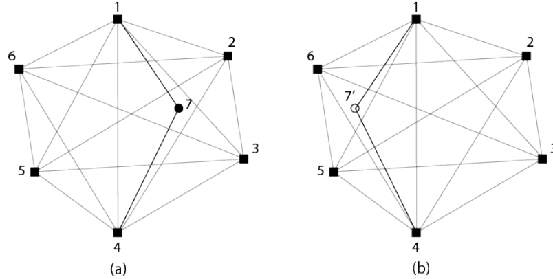
Fig. 1. Two different embeddings (a) and (b), for the same localization network that is rigid but not GGR.
