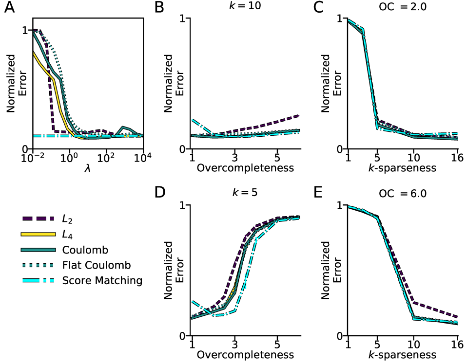
Figure 5: Coherence control costs do not all recover analysis matrices well. All ground truth analysis matrices were generated from the Soft Coherence cost and had a data dimension of 32. Color and line style legend are preserved across panels. A The normalized recovery error (see Section 3 for details) for a 2-times overcomplete analysis matrix and k = 10 as a function of the sparsity prior weight ( \lambda ). Since score matching does not have a \lambda parameter, it is plotted at a constant. B Recovery performance ( \pm s.e.m., n = 10 ) at the best value of \lambda as a function of overcompleteness at k = 10 . C Recovery performance ( \pm s.e.m., n = 10 ) at the best value of \lambda as a function of k -sparseness at 2-times overcompleteness. D , E Same plots as B and C at a point where methods do not perform as well: k = 5 and 6-times overcomplete. In B-E , the L_4 , Coulomb, and Flattened Coulomb lines are largely overlapping.
