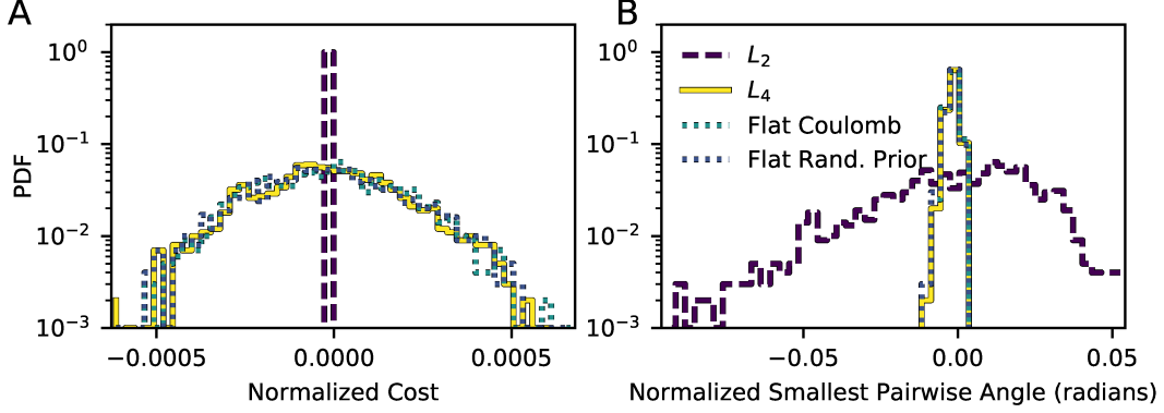
Figure C3: Local minima and saddle points do not impede optimization. A The distribution of the mean-centered final cost values normalized by the average cost value at initialization over 1000 uniform n -sphere initializations. B The distribution of the mean-centered final smallest pairwise angles over 1000 uniform n -sphere initializations.
