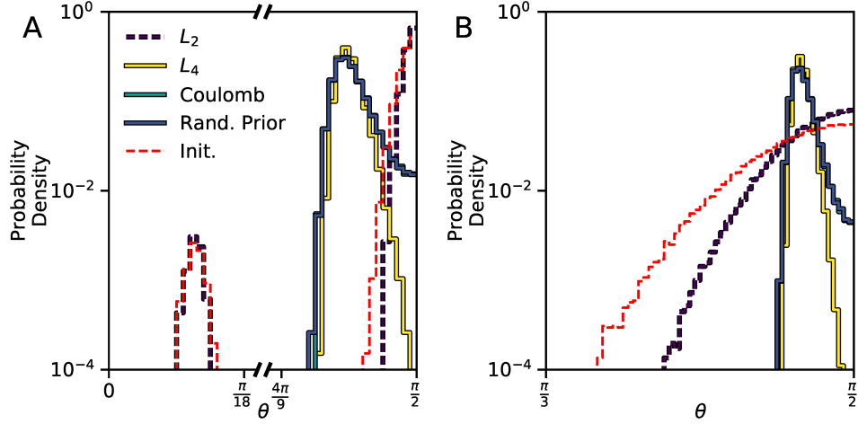
Figure 2: Coherence control costs have minima with varying coherence which can depend on initialization. Color legend is preserved across panels. For both panels a 2 times overcomplete dictionary with a data dimension of 32 was used and the distributions are averaged across 10 random initializations. A Distribution of pairwise angles (log scale) obtained by numerically minimizing a subset of the coherence cost functions for the pathological dictionary initialization. Red dotted line indicates the initial distribution of pairwise angles. Note that the horizontal axis is broken. B Angle distributions obtained through optimization from a uniform random dictionary initialization. Note that the horizontal axis only includes the range from \frac{\pi}{3} to \frac{\pi}{2} . In both plots, the Coulomb and Random Prior lines are almost entirely overlapping.
