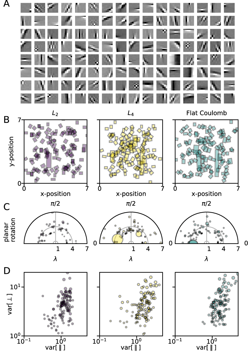
Figure 7: All coherence costs learn a dictionary that approximately tiles the space of Gabor Filters. A Dictionary learned using the L_4 cost on 8-by-8 natural image patches. B Distributions of locations, envelope scales, and rotations. Rectangle position: center of Gabor fit in pixel coordinates, rectangle rotation: planar-rotation of the Gabors, rectangle shape: envelope width parallel and perpendicular to the oscillation axis. C Distributions of rotations, log-wavelengths ( \lambda ), and envelope widths. Polar plots of planar-rotation angle and log-spatial wavelength of the Gabors. Marker size scales with geometric mean of envelope widths. D Distributions of envelope scales and log-wavelengths. Log-scale plot of envelope widths-squared parallel and perpendicular to the oscillation axis of the Gabors. Circle size scales with log-wavelength.
