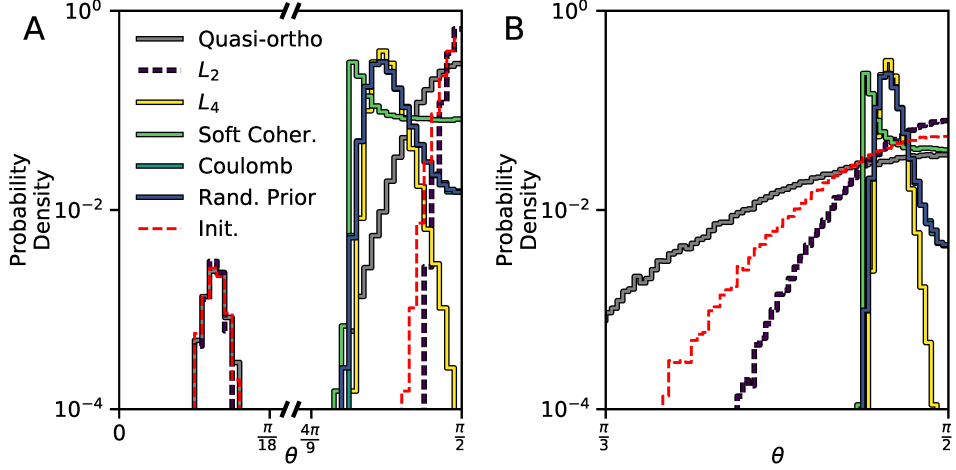
Figure C1: Coherence control costs have minima with varying coherence which can depend on initialization. Color legend is preserved across panels. For both panels a 2 times overcomplete dictionary with a data dimension of 64 was used. A Distribution of pairwise angles (log scale) obtained by numerically minimizing a subset of the coherence cost functions for the pathological dictionary initialization. Red dotted line indicates the initial distribution of pairwise angles. Note that the horizontal axis is broken at 10 and 80 degrees. B Angle distributions obtained (as in A ) from a uniform random dictionary initialization. Note that the horizontal axis only includes \frac{\pi}{3} to \frac{\pi}{2} .
