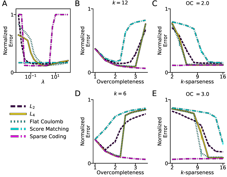
Figure 4: Coherence control costs do not all recover mixing matrices well. All ground truth mixing matrices were generated from the Soft Coherence cost and had a data dimension of 32. Color and line style legend are preserved across panels. A The normalized recovery error (see Section 3 for details) for a 2-times overcomplete mixing matrix and k = 12 as a function of the sparsity prior weight ( \lambda ). Since score matching does not have a \lambda parameter, it is plotted at a constant. B Recovery performance ( \pm s.e.m., n = 10 ) at the best value of \lambda as a function of overcompleteness at k = 12 . C Recovery performance ( \pm s.e.m., n = 10 ) at the best value of \lambda as a function of k -sparseness at 2-times overcompleteness. D , E Same plots as B and C at a point where methods do not perform as well: k = 6 and 3-times overcomplete. In B-E , the L_4 and Flattened Coulomb lines are largely overlapping.
