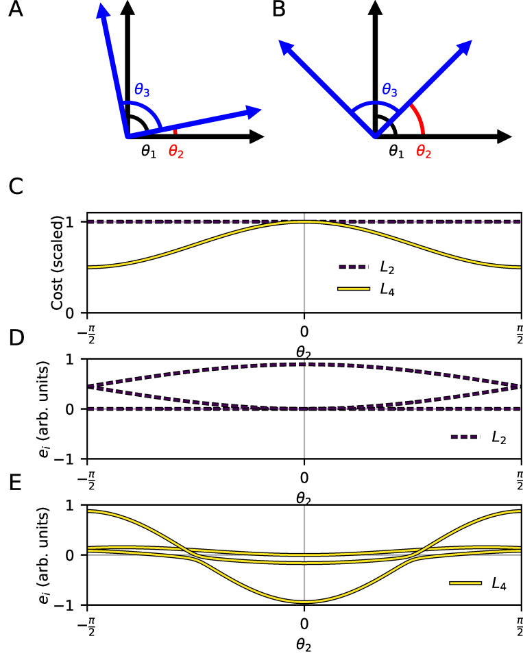
Figure 1: Structure of the pathological global minimum in the L_2 cost which the L_4 cost corrects. In A and B , each arrow represents a dictionary element in a 2-times overcomplete dictionary in a 2-dimensional space. A A dictionary with high coherence which has the same value of the cost as the dictionary in B for any \theta_2 including the pathological solution \theta_2 \rightarrow 0 . B A dictionary with low coherence. C The L_2 and L_4 costs are plotted at \theta_1 = \theta_3 = \pi/2 as a function of \theta_2 . The costs have been scaled so that their maximum value is 1. D The eigenvalues of the L_2 cost at \theta_1 = \theta_3 = \pi/2 as a function of \theta_2 scaled between -1 and 1. E The eigenvalues of the L_4 cost at \theta_1 = \theta_3 = \pi/2 as a function of \theta_2 scaled between -1 and 1.
