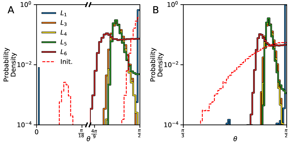
Figure C2: Coherence control costs based on powers of the difference between the Gram matrix and the identity matrix have highest coherence for powers 4 and 5. A Distribution of pairwise angles (log scale) obtained by numerically minimizing power-based coherence cost functions for the pathological dictionary initialization. Red dotted line indicates the initial distribution of pairwise angles. Note that the horizontal axis is broken at 10 and 80 degrees. B Angle distributions obtained (as in A ) from a uniform random dictionary initialization. Note that the horizontal axis only includes 65 to 90 degrees.
