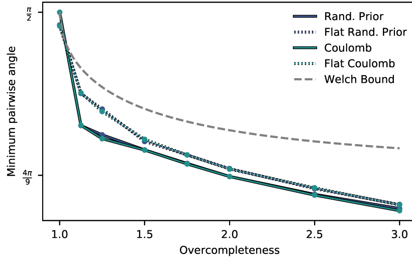
Figure C6: Quadratic terms dominate the minima of coherence control costs as a function of overcompleteness. The median minimum pairwise angle (arccosine of coherence) across 10 initializations is plotted as a function of overcompleteness for a dictionary with a data dimension of 32. The largest possible value (Welch Bound) is also shown as a function of overcompleteness.
