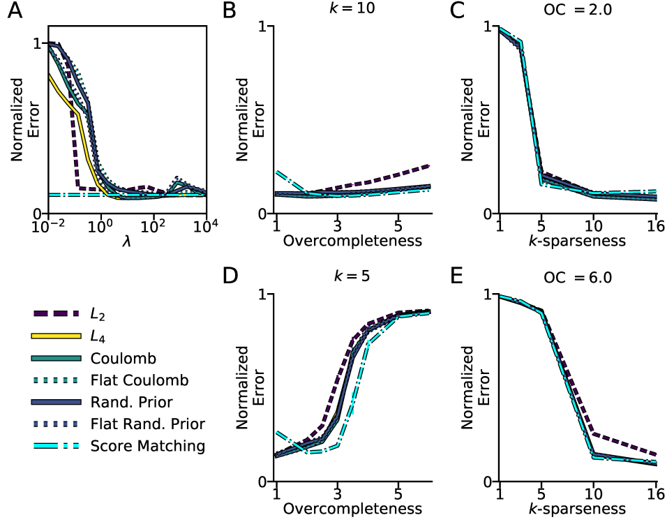
Figure C5: Coherence control costs do not all recover analysis matrices well. All ground truth analysis matrices were generated from the Soft Coherence cost and had a data dimension of 32. Color and line style legend are preserved across panels. A The normalized recovery error (see Section 3 for details) for a 2-times overcomplete analysis matrix and k = 10 as a function of the sparsity prior weight ( \lambda ). Since score matching does not have a \lambda parameter, it is plotted at a constant. B Recovery performance ( \pm s.e.m., n = 10 ) at the best value of \lambda as a function of overcompleteness at k = 10 . C Recovery performance ( \pm s.e.m., n = 10 ) at the best value of \lambda as a function of k -sparseness at 2-times overcompleteness. D, E Same plots as B and C at a point where methods do not perform as well: k = 5 and 6-times overcomplete. In B-E , the L_4 , Coulomb, Flattened Coulomb, Random, and Flattened Random lines are largely overlapping.
