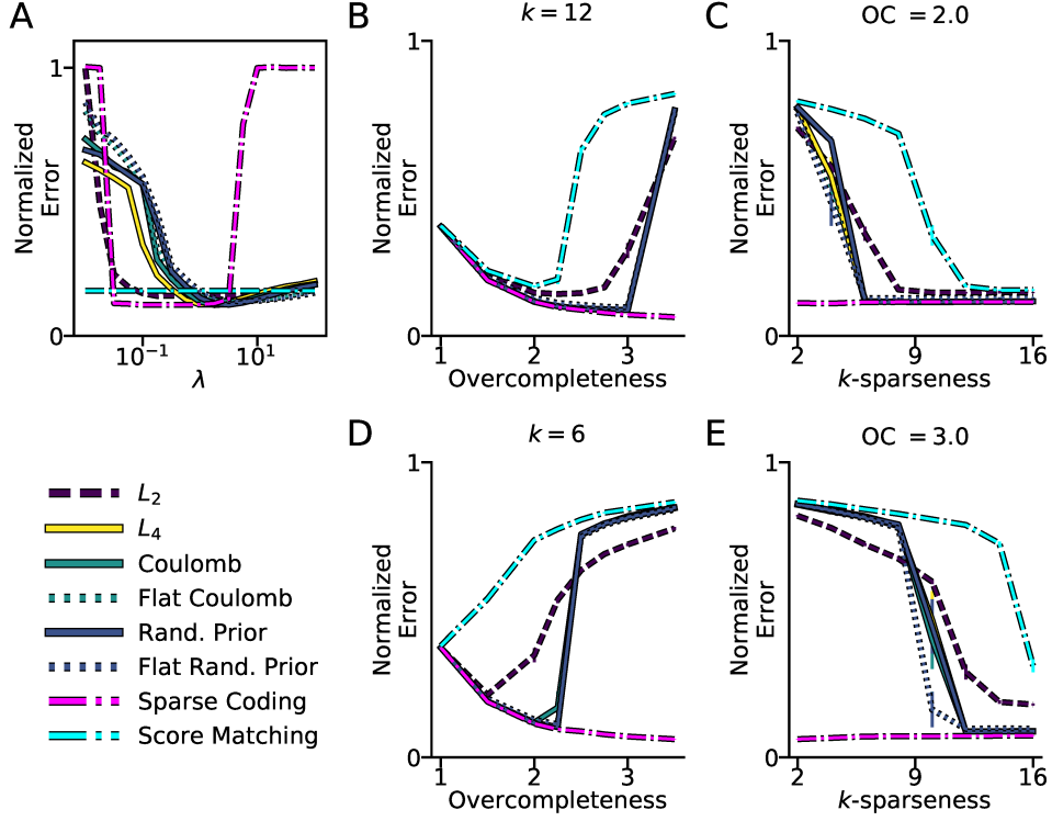
Figure C4: Coherence control costs do not all recover mixing matrices well. All ground truth mixing matrices were generated from the Soft Coherence cost and had a data dimension of 32. Color and line style legend are preserved across panels. A The normalized recovery error (see Section 3 for details) for a 2-times overcomplete mixing matrix and k = 12 as a function of the sparsity prior weight ( \lambda ). Since score matching does not have a \lambda parameter, it is plotted at a constant. B Recovery performance ( \pm s.e.m., n = 10 ) at the best value of \lambda as a function of overcompleteness at k = 12 . C Recovery performance ( \pm s.e.m., n = 10 ) at the best value of \lambda as a function of k -sparseness at 2-times overcompleteness. D, E Same plots as B and C at a point where methods do not perform as well: k = 6 and 3-times overcomplete. In B-E , the L_4 , Coulomb, Flattened Coulomb, Random, and Flattened Random lines are largely overlapping.
