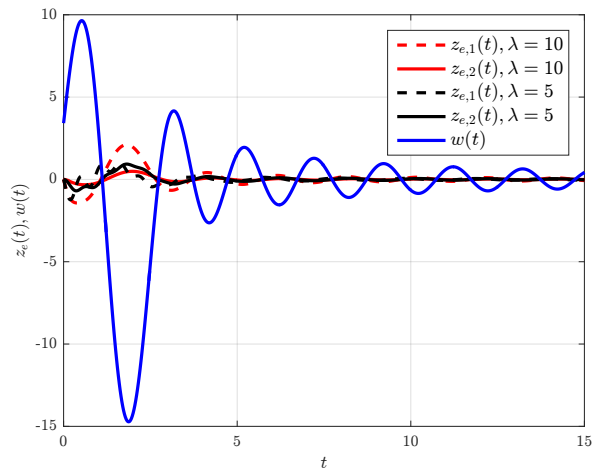
Fig. 2: For Example 2: Time evolution of z_e(t) and w(t) for \lambda = 5, 10 where w(t) is generated by damped sinusoidal functions.
