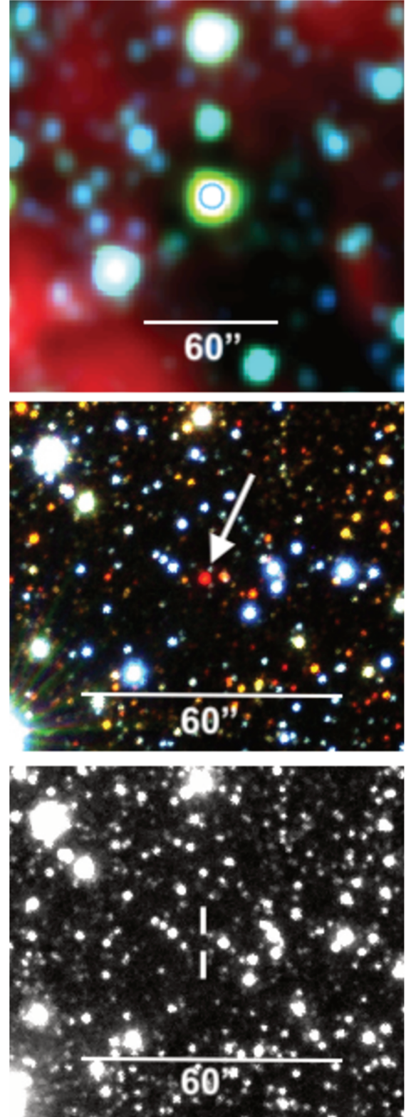
Figure 3. Finder images (equatorially oriented). (Top:) 3 \times 3' WISE 3-colour image showing VVV-WIT-01 in 2010, marked with a blue circle (blue: 3.3 \mu m, green: 4.6 \mu m, red: 12 \mu m). The green colour is due to high extinction and emission from warm circumstellar matter. (Middle:) 90 \times 80'' VVV 3-colour image (blue: J, green: H, red: K_s ) from March 2010. VVV-WIT-01 is the very red star at the centre, with additional red YSO candidates adjacent. (Bottom:) K_s stacked image made from all VVV images of the field in 2011. The transient was no longer detected.
