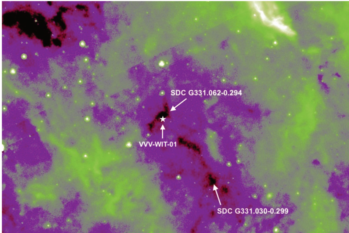
Figure 5. Spitzer /GLIMPSE 8\,\mu\text{m} 8\times 6' false colour image of the IRDCs in the VVV-WIT-01 field, with equatorial orientation. This image was taken in 2004, before the transient event (marked with a white star) in SDC G331.062–0.294. We see that this IRDC is part of a larger dark region that includes SDC G331.030–0.299. The bright diffuse 8\,\mu\text{m} background emission (green or white areas) is typical of the mid-plane of the inner Milky Way. The white area at the top right is the HII region IRAS 16067-5145 at d \approx 7.4 kpc, see text.
