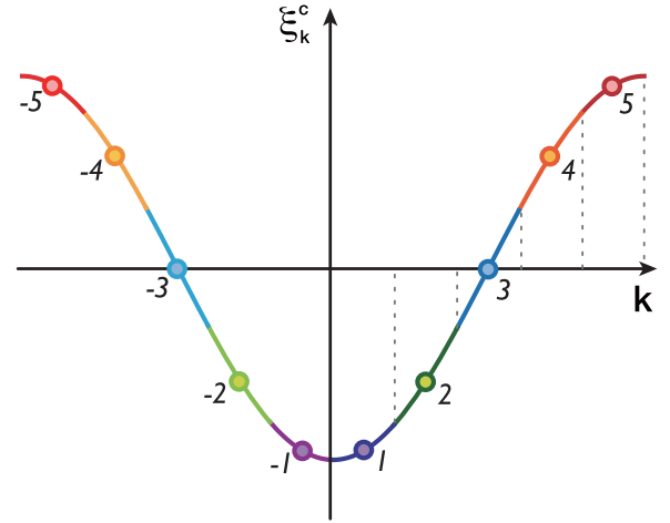
FIG. 3. Patching scheme for the functional renormalization group.
