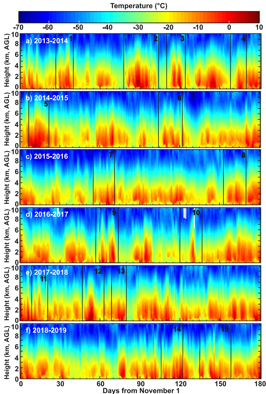
FIG. 2. Contour plots of vertical profiles of temperature (in ^{\circ}\text{C} ) obtained from twice daily DOE ARM NSA site radiosondes for the six winter seasons from 2013/14 through 2018/19. The black boxes indicate the 15 intrusions of warm, moist air analyzed in the study.
