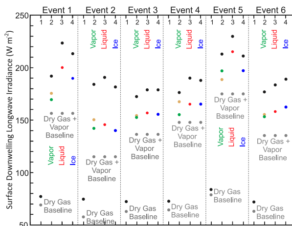
FIG. 10. Results of the analysis for the first six intrusion events. The baseline irradiances for the dry gas are indicated by the lower gray dots, whereas those for the dry gas together with water vapor are represented by the upper gray dots. The black dots just above the dry gas baseline values represent the increase in the surface downwelling longwave irradiance that resulted from temperature increases of the dry gas during the intrusion event. The vertical distance between the dry gas and dry gas plus water vapor baselines (i.e., the gray dots within an intrusion event) represents the increase in surface downwelling longwave irradiance as a result of adding the baseline amount of water vapor to the baseline amount of dry gas for the intrusion event. The gold dots indicate the average surface downwelling longwave irradiance over the intrusion event as a result of temperature changes above their baseline value with water vapor and pressure fixed to their baseline values. The green, red, and blue dots indicate the average surface downwelling longwave irradiance over the intrusion event as a result of water vapor, liquid water, or ice water changes, respectively, above their baseline dry gas plus water vapor values with pressure and temperature held fixed. The black dots indicate the average surface downwelling longwave irradiance over the intrusion event as a result of temperature and either water vapor, liquid water, or ice water changes above their baseline dry gas plus water vapor values with now only pressure held fixed. The vertical distances from the gray dots representing the dry gas plus water vapor baseline to the green, red, and blue dots for each constituent represent the efficacy of the constituent alone in elevating the surface downwelling longwave irradiance above its baseline value during the intrusion event. The vertical distances from the green, red, and blue dots to the black dots above them represent the additional increase in surface downwelling longwave irradiance from a constituent as a result of both constituent and temperature changes during the intrusion event. These results are presented in tabular format within Table 2 for all 15 intrusion events.
