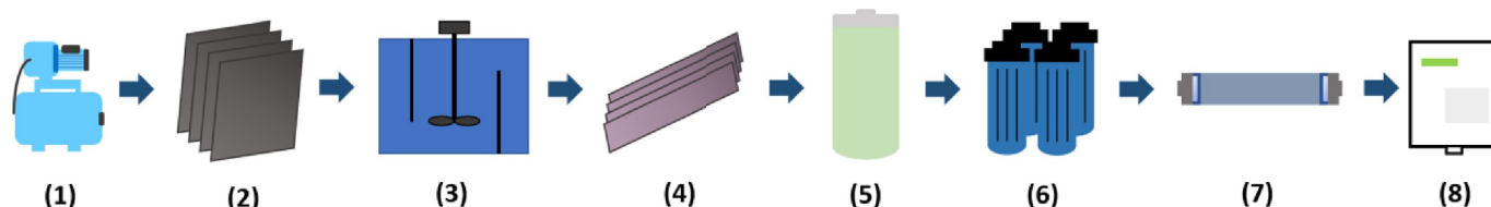
Fig. 3. Schematic representation of the treatment process at the Dhaphdapi pilot plant: 1) raw water pump, 2) ECAR reactors, 3) flocculation chamber, 4) tube settler, 5) rapid sand filter, 6) micron filters, 7) ultraviolet disinfection system, 8) automatic dispensing unit.
