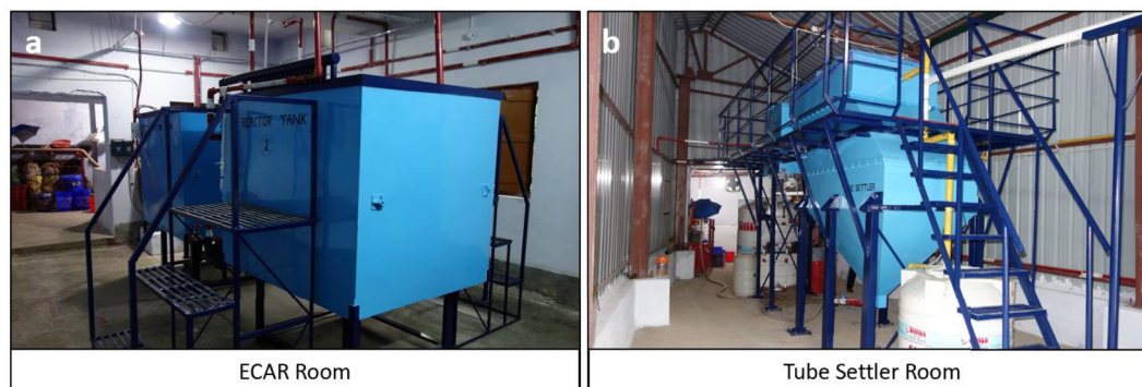
Fig. 2. Digital photographs of the 10,000 LPD capacity pilot plant at Dhaphdapi High School. a) ECAR Room: Contains the two ECAR reactors in which electrolysis occurs b) Tube Settler Room: Contains the tube settler, flocculation chamber, and subsequent tertiary treatment systems for particle separation.
