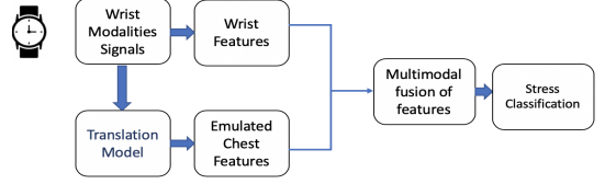
Fig. 2. Stress detection using wrist sensors with translated features for chest
