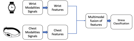
Fig. 1. Stress detection pipeline using both wrist and chest sensors
