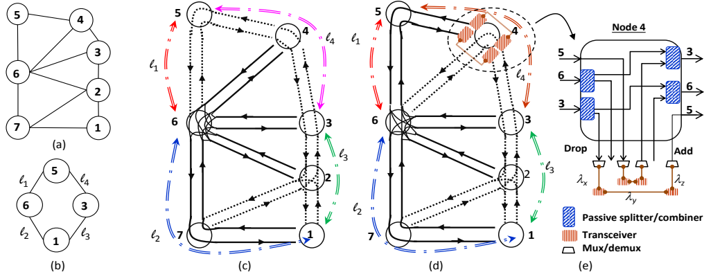
Fig. 2. (a) 7-node German network, (b) virtual network, (c) and (d) show two fiber tree establishments (highlighted by solid and dotted lines in each of the figures) and SVNMs of the logical topology (in (c) a SVNMs is possible without the use of inter-tree transceivers while in (d) the deployment of inter-tree transceivers is necessary to guarantee a SVNMs), and (e) architecture of node 4 showing position of inter-tree transceivers deployed
