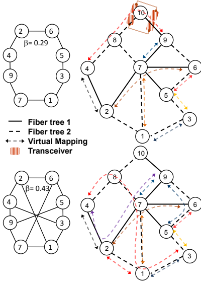
Fig. 4. Two SVNМs for Surv-FON*
