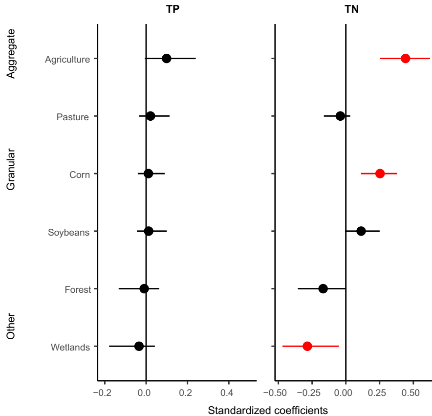
FIG. 2. Population-level slope estimates ( \mu_j ) for the effect of watershed land-use cover on lake total nitrogen (TN) and total phosphorus (TP) from six candidate models. Values shown are posterior medians (filled circles) and 95% credible intervals (solid lines). Also shown is a comparison to a zero effect (solid vertical line). Values that do not overlap zero are shaded in red. Coefficient estimates are reported relative to standardized predictor variables centered at zero with unit variance.
