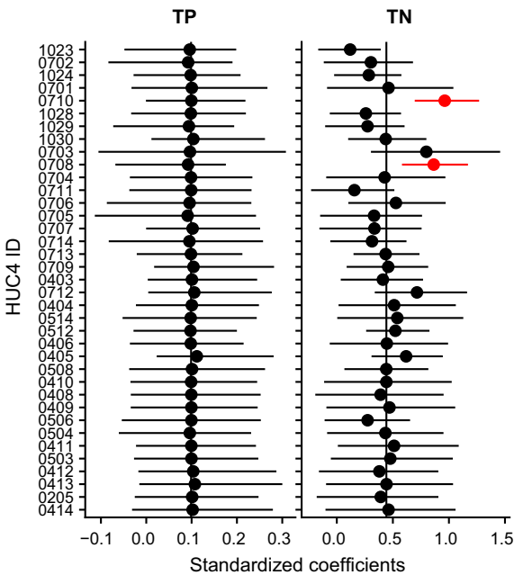
FIG. 4. Effect of watershed land use ( \gamma ) for individual regions in the top-ranked lake N and P models. Values shown are posterior medians (solid circles) and 95% credible intervals (solid lines) for individual hydrologic units (HUC4s) ordered from top to bottom according to longitude (west to east). Also shown is a comparison to a zero effect (solid vertical line). Values that are different from the population level effect are shaded in red.
