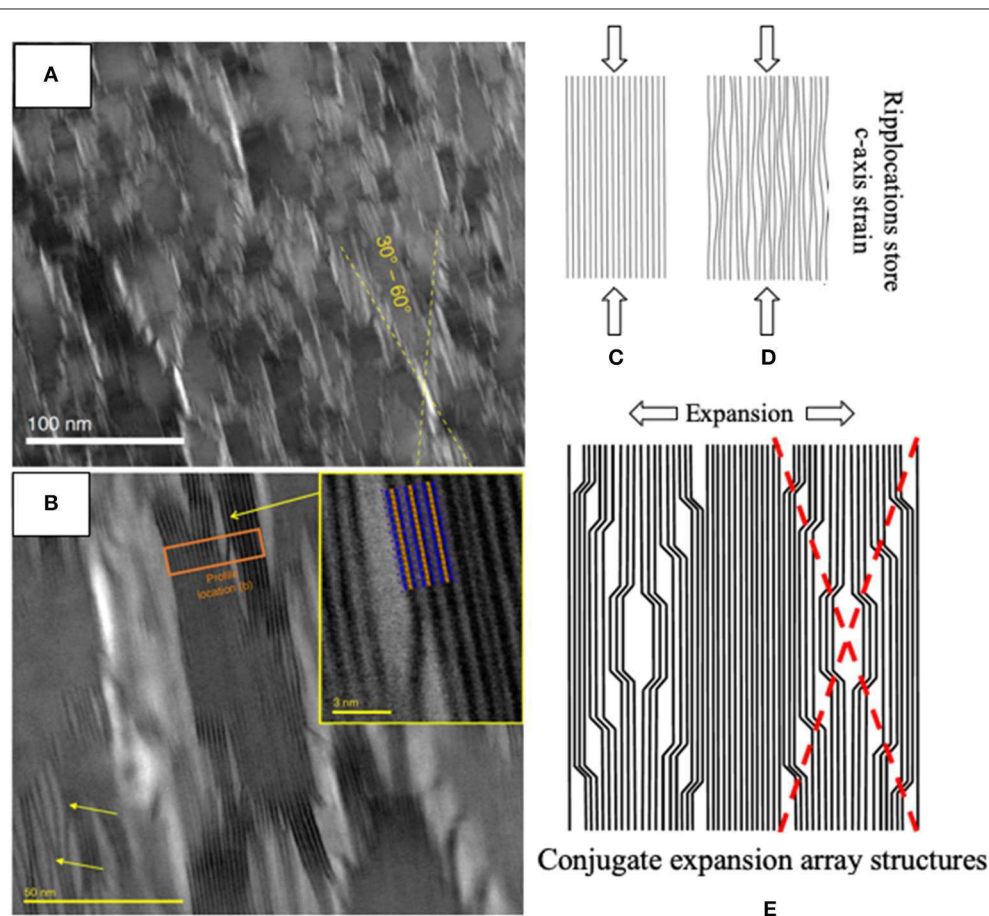
FIGURE 8 | (A) Transmission electron microscope micrographs of a natural biotite. Bright streaks are revealed to be up to 60 Å wide, lozenge-shaped lattice expansion, or delamination, structures of biotite basal planes. The acute angles of these diamonds measure between 30° and 60°. (B) Lattice curvature and interlayer expansion. Inset is a higher magnification image of the orange rectangle shown in micrograph emphasizing atomic nature of the deformation. (C) Perfect layers subjected to compression. (D) Ripplifications store c -axis strain that, when released, results in, (E) Conjugate arrays of expansion structures and delaminations observed (Aslin et al., 2019). Reproduced under the Creative Commons CC BY license.
