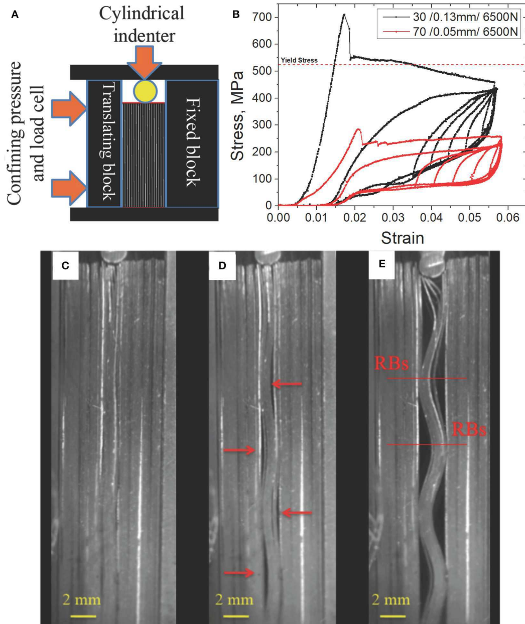
FIGURE 3 | (A) Setup used to study ripplacations in layered systems (Gruber et al., 2016). (B) Typical stress-strain curves of thin steel sheets. Difference between the two curves is in the thickness of the deck and the thickness of the layers in each deck. Confining pressure was the highest used here 6500 N (Badr et al., 2020). Drop in maximum stress coincided with buckling and nucleation of RBs. Still frames of movie of loading steel sheets, (C) initial configuration with cylindrical indenter oriented into the page at top. (D) Nucleation of RBs at maximum stress in b. Note delaminations. (E) Same as (D) but at maximum penetration depth. RBs, precursors of kink boundaries, are defined as locus of regions with maximum curvature, i.e., crests of standing waves. Upon removal of the load, the configuration returns to one quite similar to that shown in (A) . Said otherwise the process is reversible.
