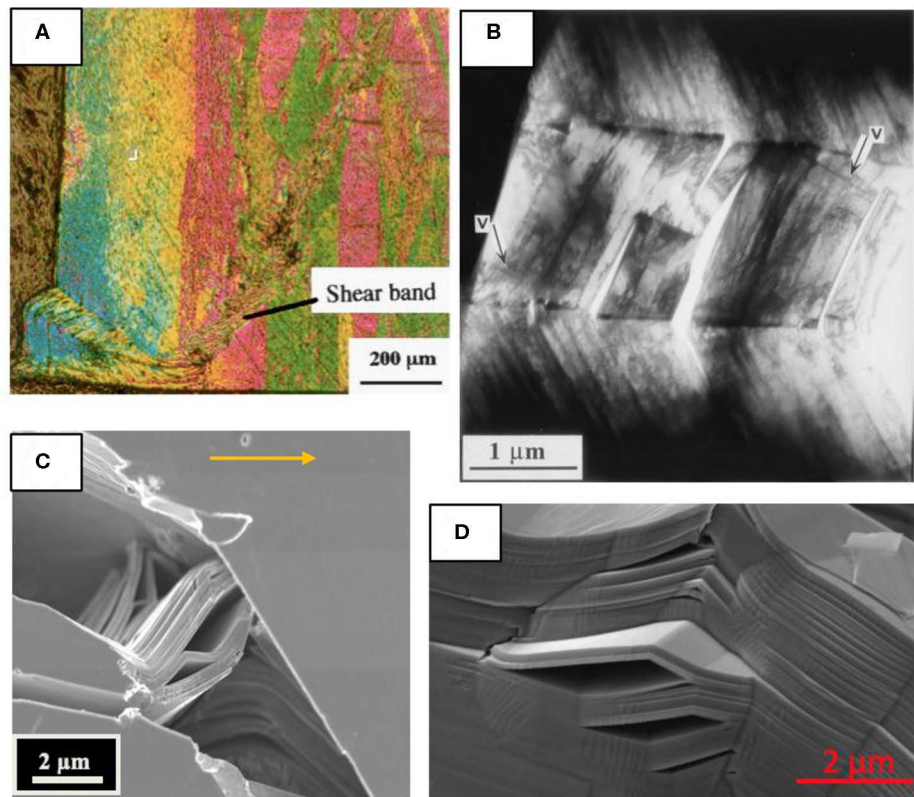
FIGURE 1 | Kink band, KB, formation in the MAX phase \text{Ti}_3\text{SiC}_2 at various scales. (A) Kink band formed at edge of a 2 mm cube wherein the basal planes were highly oriented vertically (Barsoum and El-Raghy, 1999). (B) KB in TEM, (Barsoum et al., 1999). (C) Field-emission scanning electron microscope, SEM, image of a bridged crack in a coarse-grained \text{Ti}_3\text{SiC}_2 microstructure (Gilbert et al., 2000). Heavily deformed lamella bridge the crack and significant amounts of delamination and bending/kinking are observed. Such processes are highly unusual in ceramic systems and account for the high plateau fracture toughness values measured. Arrow indicates direction of crack propagation. (D) KBs and concomitant delaminations of a solid bridge between pores (Sun et al., 2005) (A,B) reproduced with permission from Metallurgical and Materials Transactions A, Springer Nature. (C,D) Reproduced with permission from Scripta and Acta Materialia, Elsevier.
