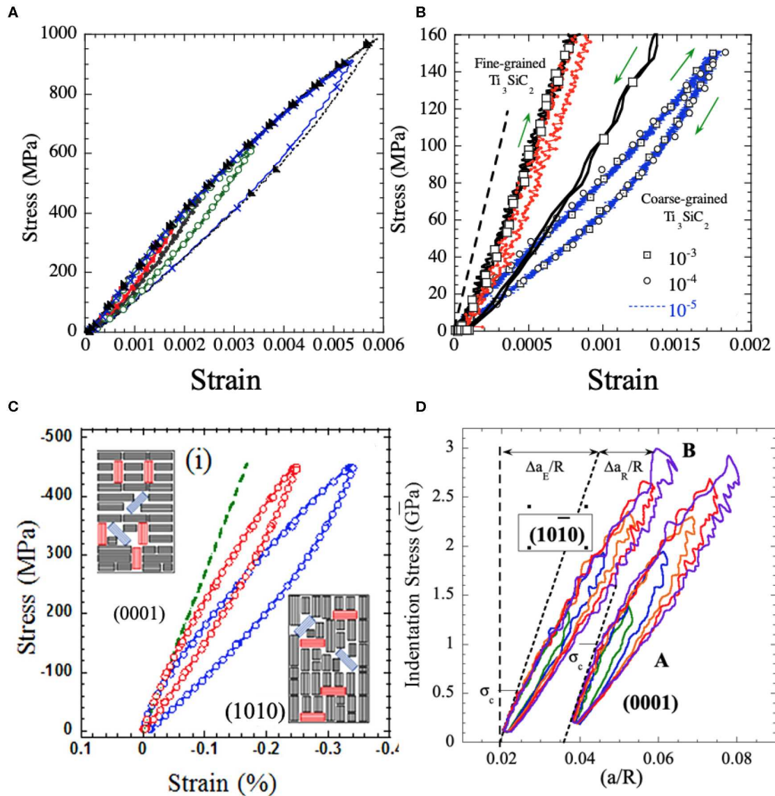
FIGURE 2 | Typical bulk cyclic compressive spontaneously reversible stress/strain loops in (A), Fine-grained, FG, \text{Ti}_3\text{SiC}_2 , (B) Same as (A) but showing dramatic difference in response between coarse-grained, CG (small blue loops), and FG samples (black and red loops). Note the blue loops comprise three different loops, obtained at three strain rates indicated. Red loop—obtained on FG sample at 250 MPa—is significantly stiffer and smaller in area than the CG loops at the same stress; Within the resolution of the measurement, the three loops at the various strain rates are identical. (C) Highly oriented polycrystalline \text{Ti}_2\text{AlC} samples where, (i) basal planes are mostly normal to the applied load (red loop) or, (ii) parallel to the applied load (blue loop) (Shamma et al., 2015). In insets, thin lines represent basal planes. Black and red rectangles represent majority and minority hard grains, respectively. Blue rectangles represent soft grains. (D) NI stress vs. a/R , where a is the contact radius and R is the indenter diameter, for basal planes loaded edge on, viz. (1010) and those loaded normal to the basal planes, viz. (0001) (Griggs et al., 2017). (C,D) Reproduced with permission from Acta Materialia, Elsevier.
