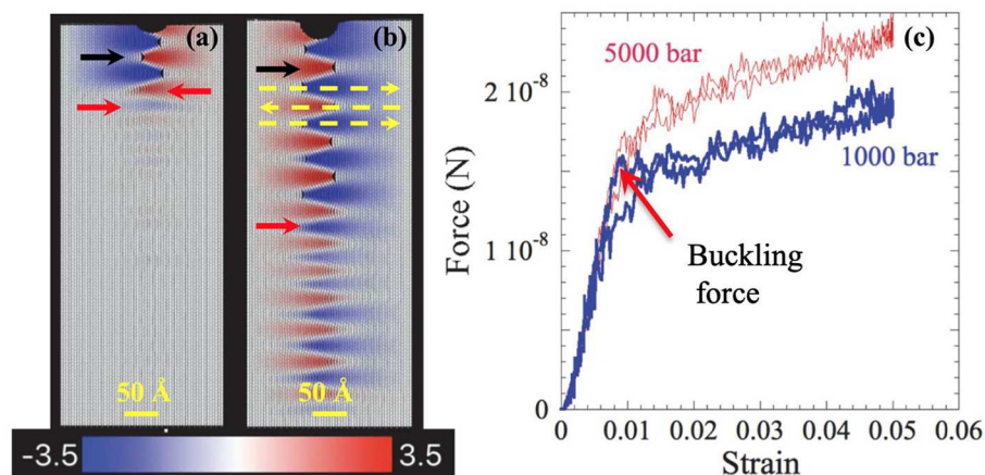
FIGURE 9 | (a) Molecular dynamics, MD, simulation of indenting graphite layers edge-on at the nucleation of the RBs. Color scale in (a) quantifies atomic motion along the z axis, in Å, to the right (blue) or left (red). (b) same as (a) , but at maximum penetration. (c) MD load vs. strain curves. Point at which the slope of the force/strain curves changes coincides with nucleation of ripplocation boundaries, RBs. Process is fully reversible (Barsoum et al., 2019). Yellow arrows denote RBs of opposite signs. Black arrows point to delaminations. Horizontal red arrows point to regions where the deformation is accommodated without delaminations. Black arrows point to delaminations.
