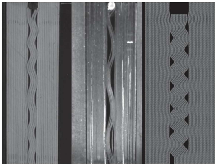
FIGURE 11 | Snapshots of RBs formed when a cylindrical indenter is loaded edge-on into plastic cards ( left ), thin steel plates ( middle ), and graphite ( right ). The latter is a result of a MD simulation. The scales are intentionally not shown.
