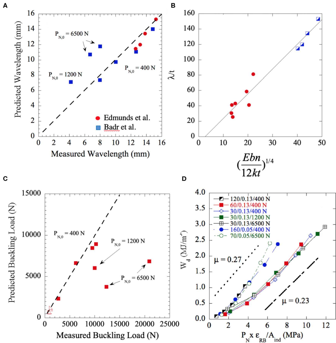
FIGURE 5 | (A) Comparison of measured and predicted wavelengths, \lambda , (B) \lambda/t vs. (Ebn/12kt)^{1/4} , (C) Comparison of measured and predicted buckling loads. (D) Plot of W_d vs. (P_N \epsilon_{RB}/A_{ind}) . Slope of these lines is proportional to the friction coefficient, \mu (Badr et al., 2020).
