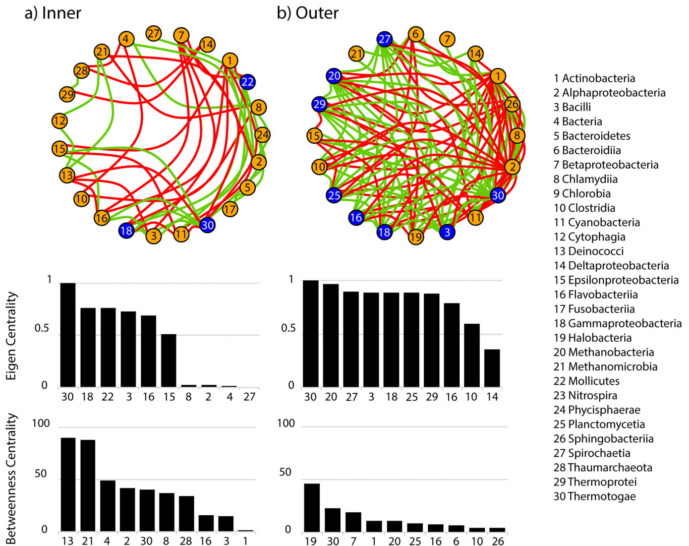
FIG 4 Network analysis of the coral SML microbiome of P. strigosa from inner (A) and outer (B) reefs. Each node represents a microbial class interconnected by positive correlations (green) and negative correlations (red) (Spearman's \rho > 0.7 ). Nodes that have an eigen centrality higher than 0.75 are highlighted in blue. The top 10 values of eigen centrality and betweenness centrality across microbial classes are graphed below each network.
