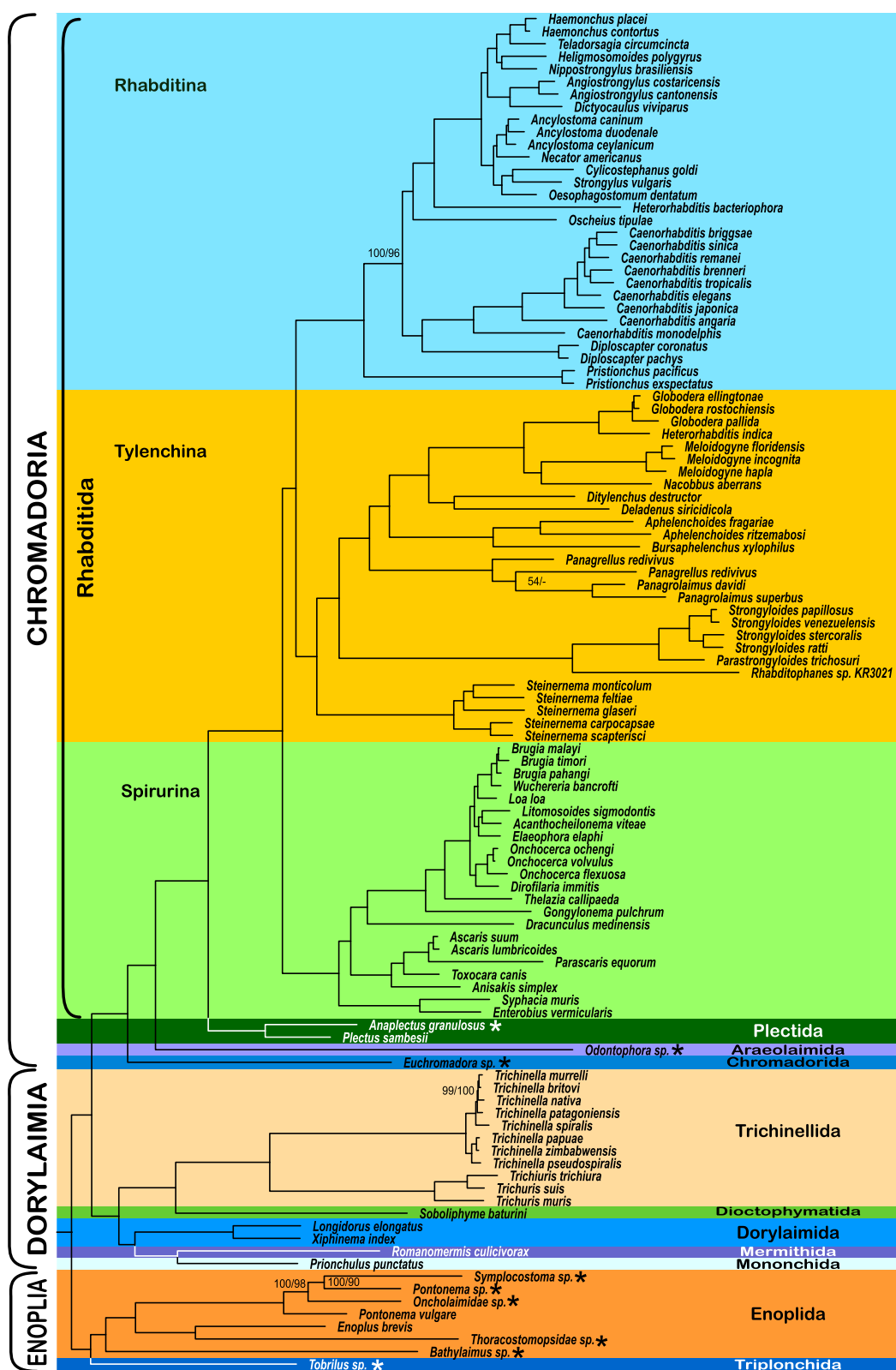
Fig. 2 Phylogeny of Nematoda based on the IQ-TREE maximum likelihood analysis of the ScaFoS dataset. IQ-TREE / RAxML bootstrap support values < 100% are shown. Newly generated transcriptomes are marked with an asterisk
