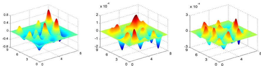
Fig. 4 Plotted on the left is a nonseparable spline signal of the form (5.17), where K = [0, 7] \times [0, 6] , and in the middle and on the right are the difference between the above signal f and the signal f_\epsilon reconstructed by the MAPSET algorithm with noise level \epsilon = 10^{-4} and the sampling set \Gamma being \Gamma_2 and \Gamma_3 in Fig. 3, respectively. The maximal amplitude errors e(\epsilon) in (5.15) are 2.4922 \times 10^{-4} (middle) and 3.8975 \times 10^{-4} (right). The reconstruction errors \min_{\delta \in [-1, 1]} \|f_\epsilon - \delta f\|_\infty are 1.9660 \times 10^{-4} (middle) and 2.9216 \times 10^{-4} (right)
