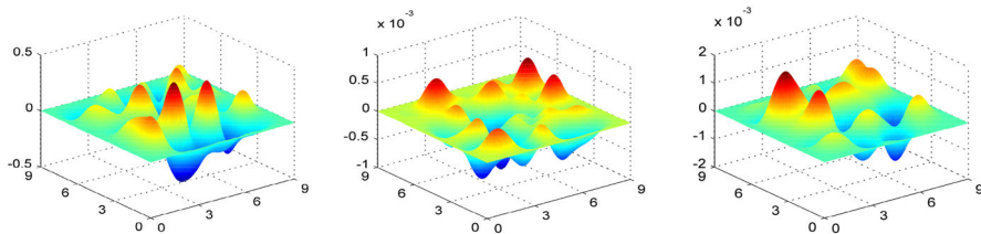
Fig. 2 Plotted on the left is a nonseparable spline signal in (5.12) with K_1 = K_2 = 7 . In the middle and on the right are the difference between the above spline signal f and the signal f_\epsilon reconstructed by the MAPSET algorithm with noise level \epsilon = 10^{-4} and sampling set \Gamma being \Gamma_0 and \Gamma_1 in Fig. 1, respectively. The maximal amplitude errors e(\epsilon) in (5.15) are 0.0014 (middle) and 0.0030 (right), and the reconstruction errors \min_{\delta \in \{-1, 1\}} \|f_\epsilon - \delta f\|_\infty are 7.2567 \times 10^{-4} (middle) and 0.0015 (right), respectively
